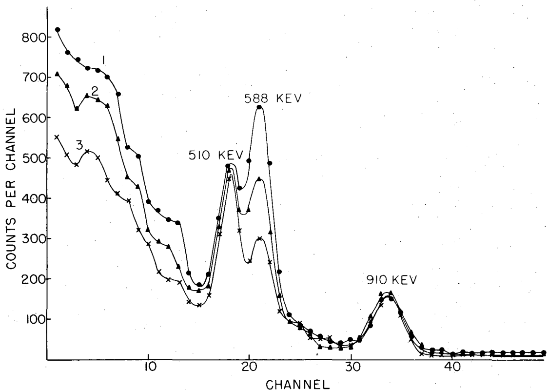
Fig. 2. Gamma spectrum of Zr^{89m} and Zr^{89} isolated from Nb^{89} after an 8-minute growth period. Curve one is a one-minute run started 8.2 minutes after an 8-minute growth period. The 588-kev gamma ray of Zr^{89m} is plainly visible. Succeeding one-minute runs show the rapid decay of this 4.4-minute activity.
