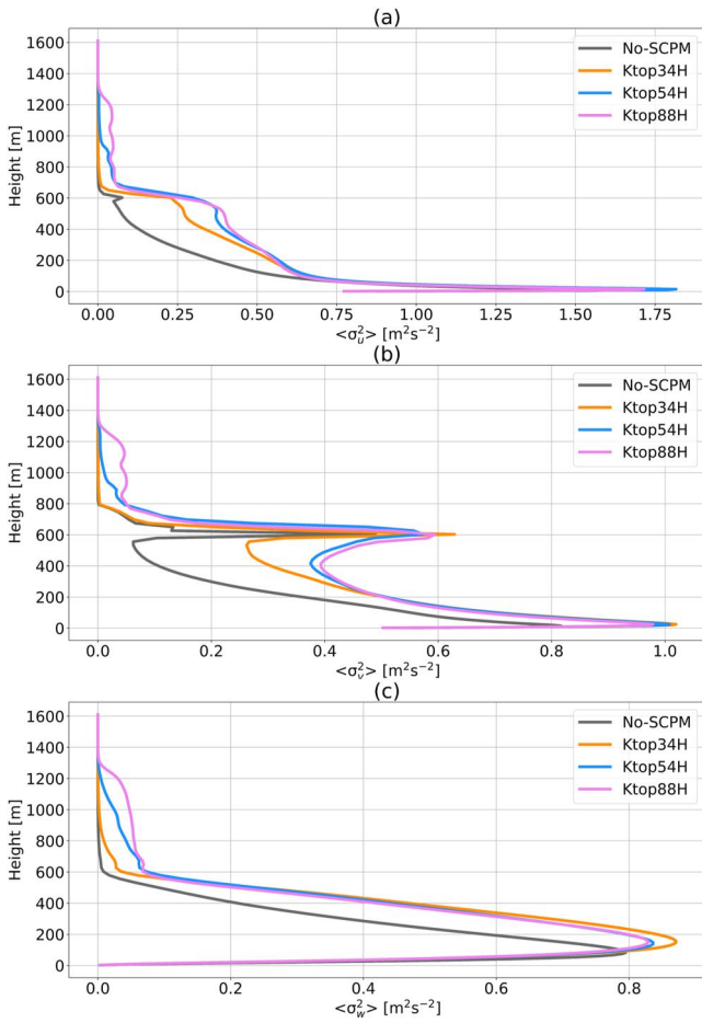
Figure 6. Area-averaged (a) \langle \sigma_u^2 \rangle , (b) \langle \sigma_v^2 \rangle , and (c) \langle \sigma_w^2 \rangle over three quarters of the domain (all y and x from 2,880 to 11,520 m) for No-SCPM, Ktop34H, Ktop54H, and Ktop88H. These results are shown from the last simulation period at 20 Z and for the top of the entire simulation inner domain up to 1,608 m. The angular brackets denote area averaging.
