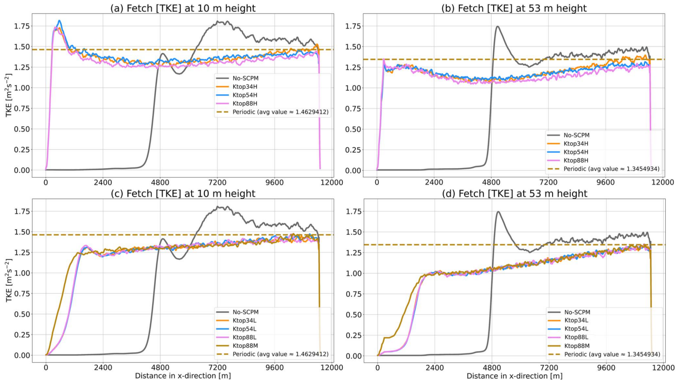
Figure 2. Fetch of Y-averaged turbulent kinetic energy (TKE) ( \text{m}^2/\text{s}^2 ), computed after applying momentum perturbation with higher, medium, and lower amplitudes as shown in (Table 1) and show fetch at (a) 10 m height for periodic, No-SCPM, and higher amplitude SCPM-M, (b) 53 m height for periodic, No-SCPM, and higher amplitude SCPM-M, (c) 10 m height for periodic, No-SCPM, and lower and medium amplitude SCPM-M, (d) 53 m height for periodic, No-SCPM, and lower and medium amplitude SCPM-M. These plots are generated for TKE that are Y-averaged over the entire inner domain.
