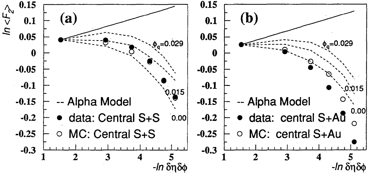
Figure 10: \ln \langle F_2 \rangle as a function of \ln(\delta\eta\delta\phi) for Alpha Model calculations (dashed lines) with slopes 0.029, 0.015 and 0.0: (a) dN/d\eta = 48 : closed (open) circles are data (Monte Carlo results) for central ^{32}\text{S}+\text{S} events; (b) dN/d\eta = 115 : closed (open) circles are data (Monte Carlo results) for central ^{32}\text{S}+\text{Au} events. In both cases the solid line represents the Alpha Model for a slope of 0.029 but without hit merging due to the finite two-track resolution. All Alpha Model calculations have been scaled vertically so that their leftmost point in the plot matches that of the data. A hit efficiency of 100% was assumed.
