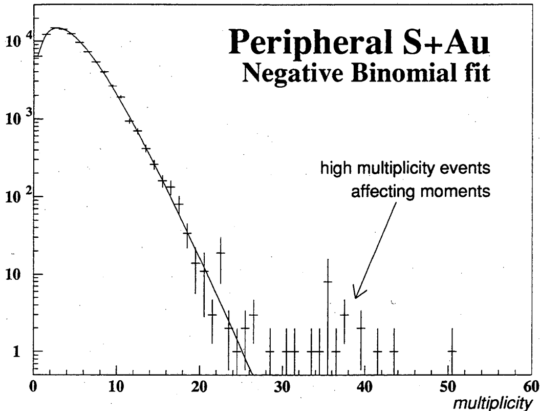
Figure 12: Multiplicity distribution for tracks within the acceptance \Delta\eta-\Delta\phi for peripheral ^{32}\text{S}+\text{Au} collisions. A negative binomial fit is also shown. The data for multiplicity \geq 30 , even though they represent only 2/10,000 of the total distribution, strongly affect the value of the higher order moments.
