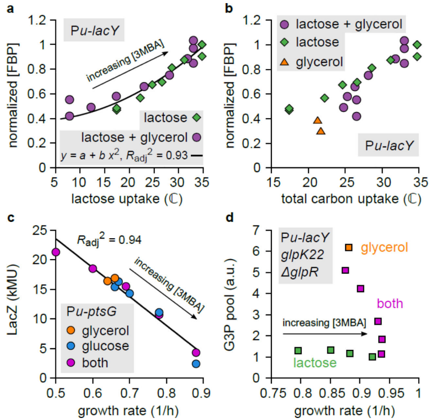
Figure 4. Glycerol uptake is regulated by two flux sensors: FBP and cAMP–Crp.
