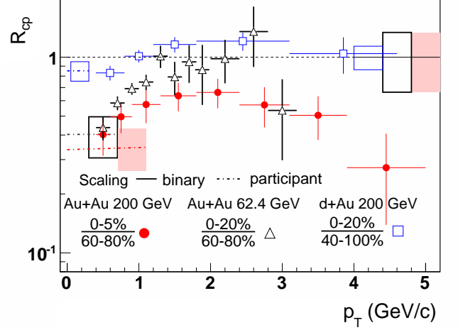
FIG. 18: (Color online) p_T dependence of the nuclear modification factor R_{cp} in Au+Au 62.4 and 200 GeV and d +Au 200 GeV collisions, where rectangular bands represent the uncertainties of binary and participant scalings (see legend). Statistical and systematic errors are included.
