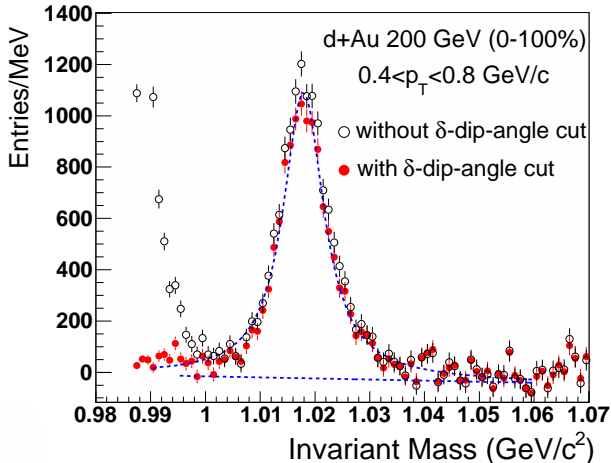
FIG. 2: (Color online) Background-subtracted invariant mass distributions at 0.4 < p_T < 0.8 GeV/c in d+Au 200 GeV collisions (0-100%) with (solid points) and without (open points) the \delta -dip-angle cut. The dashed curves show a Breit-Wigner (see the text for details) + linear background function fit to the case with the \delta -dip-angle cut.
