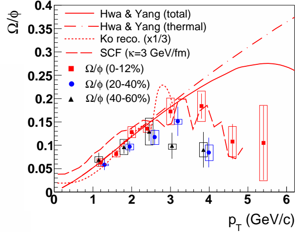
FIG. 16: (Color online) The \Omega/\phi ratio vs. p_T for three centrality bins in \sqrt{s_{NN}} = 200 GeV Au+Au collisions, where the data points for 40-60% are shifted slightly for clarity. As shown in the legend, the lines represent the results from Hwa and Yang [96], Ko et al. [97] and for SCF, Refs. [98, 99].
