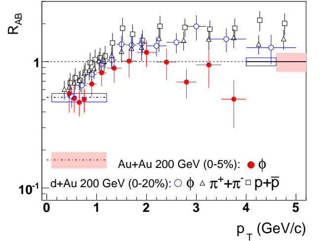
FIG. 19: (Color online) p_T dependence of the nuclear modification factor R_{AB} for \phi in Au+Au 200 GeV and d +Au 200 GeV collisions. For comparison, data points for \pi^+ + \pi^- in d +Au 200 GeV and p + \bar{p} in d +Au 200 GeV are also shown (see legend). Rectangular bands show the uncertainties of binary (solid line) and participant (dot-dash line) scalings. Systematic errors are included for \phi , \pi^+ + \pi^- and p + \bar{p} .
