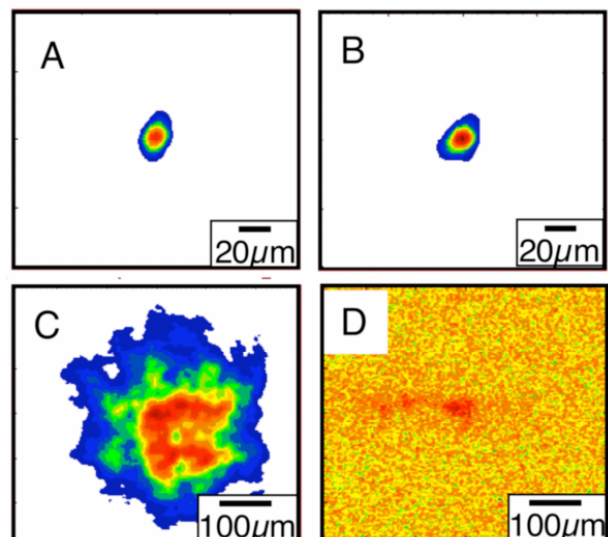
FIGURE 2. Mode images of laser propagation at 4 TW. The output image with the guide on (b) is indistinguishable from the input (a) indicating unaberrated propagation at twice P_{\text{crit}} . Unguided images show diffraction in vacuum (c) and ionization enhanced diffraction with the gas jet on (d).
