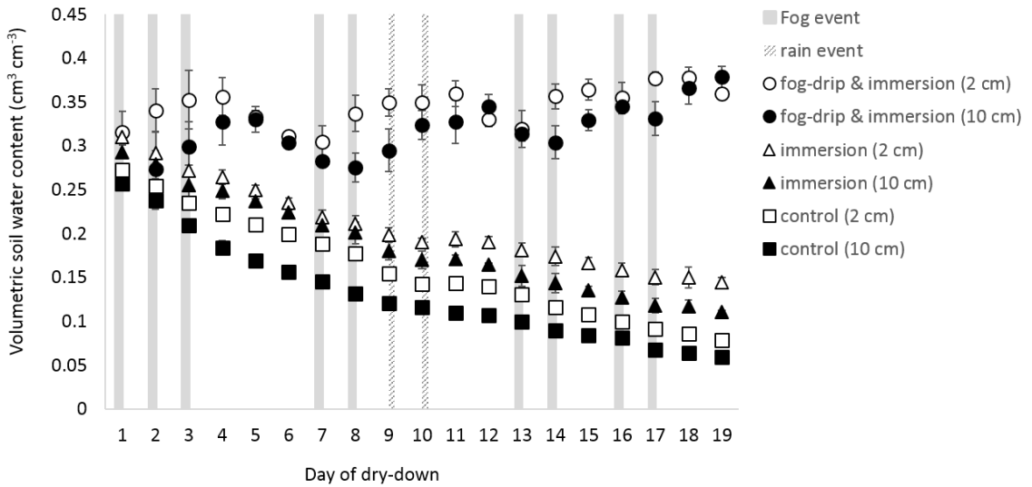
Figure 4.2. Average volumetric soil water content at 2 and 10 cm depth ( n=5 and 3 , respectively) for each treatment group during the dry-down period (circles, fog-drip & immersion; triangles, fog immersion; squares, control). Grey bars represent simulated nighttime fog events. Average soil moisture among treatment groups and control were significantly different from each other at each time point based on pairwise comparisons ( p<0.001 ). Within each group, soil moisture at 2 and 10 cm was significantly different from day 1 through the dry-down period ( p<0.001 ). Error bars represent standard error of the mean.
