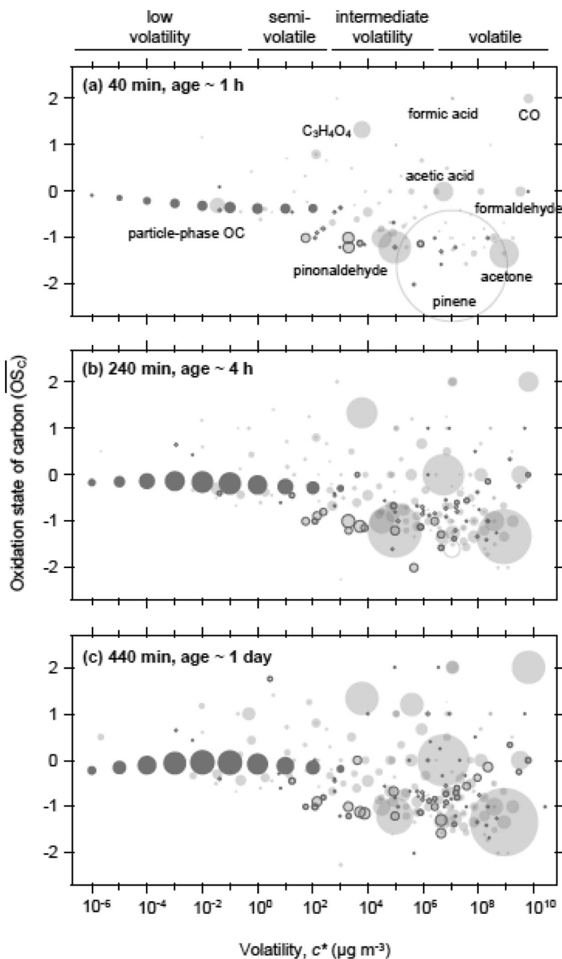
Figure 2. Chemical characterization of carbon measured in the photooxidation of \alpha -pinene in terms of \overline{OS}_C and c^* , commonly used for simplified representation of atmospheric organic carbon. These measurements illustrate the highly dynamic nature of the chemical system. Circle area is proportional to carbon concentration. Hollow: \alpha -pinene, light gray: gas-phase species, dark gray: pOC, shown at average \overline{OS}_C of each volatility bin measured by TD-AMS. Gas-phase species containing nitrate groups (defined as containing nitrogen and 3 oxygen atoms) are outlined. Distributions are provided after approximately (a) 1 hour, (b) 4 hours,
