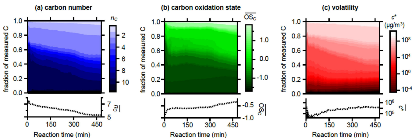
Figure 3. Distribution of key chemical properties of gas- and particle-phase products during the photooxidation of \alpha -pinene: (a) number of carbon atoms, n_C , (b) oxidation state of carbon, \overline{OS}_C , and (c) volatility in terms of saturation concentration, c^* , each denoted by the color scale shown. The properties of only the measured oxidation products (and not of the \alpha -pinene precursor or the “unmeasured” carbon) are shown; the plots in which \alpha -pinene is included is provided in Supplementary Fig. 6. Evolution of distributions and carbon-weighted averages of each property (bottom panels) demonstrate several general trends in atmospheric oxidation: initial formation of pOC and lightly-oxygenated moderately-volatile products, followed by fragmentation of gases to yield small oxygenated compounds.
