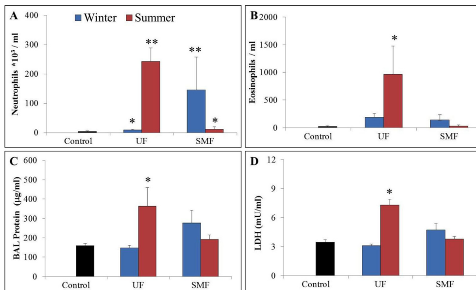
Fig. 2. Pulmonary response to summer and winter vehicle emissions. (A) Neutrophils, (B) Eosinophils, (C) BALF protein, and (D) LDH, expressed as mean \pm SEM, recovered in BALF 24 h post-exposure to 50 \mu\text{g} winter (blue) or summer (red) UF or SMF vehicle emissions. Asterisks (* p < 0.05 ; ** p < 0.0001 ) indicate significant differences from control (black bar). (For interpretation of the references to color in this figure legend, the reader is referred to the web version of this article.)
