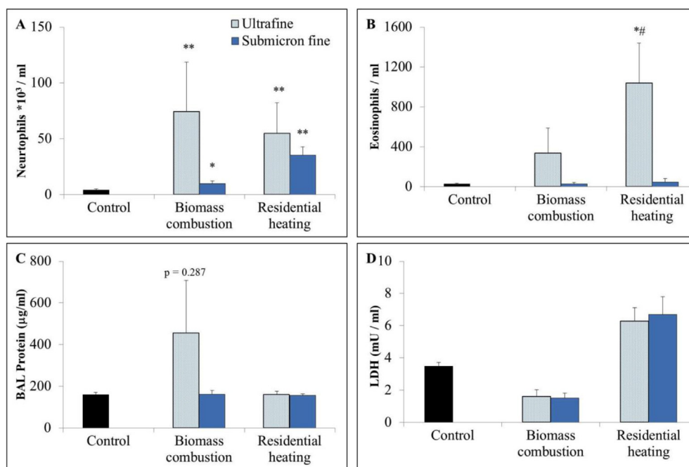
Fig. 6. Pulmonary response to winter biomass combustion emissions related to residential heating. (A) Neutrophils, (B) Eosinophils, (C) BALF protein, and (D) LDH, expressed as mean \pm SEM, recovered in BALF 24 h post-exposure to 50 \mu\text{g} or summer UF (light blue) or SMF (dark blue) biomass combustion and residential heating PM. Asterisks (*p < 0.05; **p < 0.0001) indicate significant differences from control (black bar); # indicates significantly different from the SMF fraction from the same source. (For interpretation of the references to color in this figure legend, the reader is referred to the web version of this article.)
