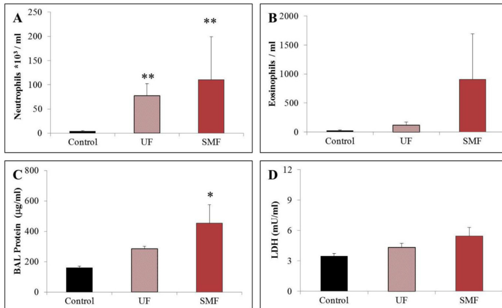
Fig. 4. Pulmonary response to unknown metals-rich source. (A) Neutrophils (B) Eosinophils (C) BALF protein, and (D) LDH, expressed as mean \pm SEM, recovered in BALF 24 h post-exposure to 50 \mu g summer UF (light red) or SMF (dark red) metal-rich PM. Asterisks (* p < 0.05; ** p < 0.0001) indicate significant differences from control (black bar); # indicates significantly different from the SMF fraction as indicated by brackets. (For interpretation of the references to color in this figure legend, the reader is referred to the web version of this article.)
