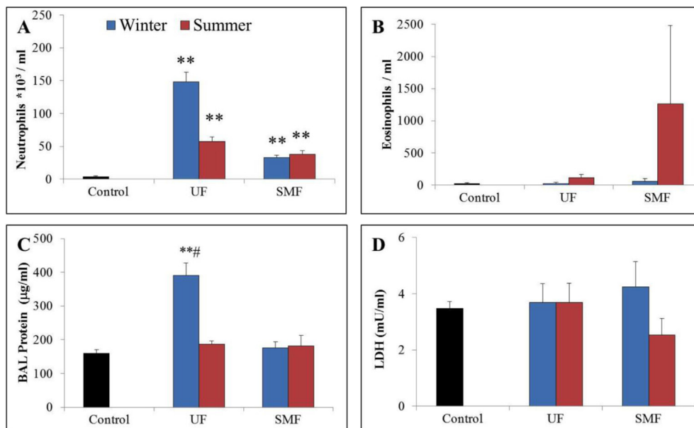
Fig. 5. Pulmonary response to summer and winter nocturnal inversion PM. (A) Neutrophils, (B) Eosinophils, (C) BALF protein, and (D) LDH, expressed as mean \pm SEM, recovered in BALF 24 h post-exposure to 50 \mu g winter (blue) or summer (red) UF or SMF nocturnal inversion PM. Asterisks (* p < 0.05; ** p < 0.0001) indicate significant differences from control (black bar); # indicates significantly different from the SMF fraction. (For interpretation of the references to color in this figure legend, the reader is referred to the web version of this article.)
