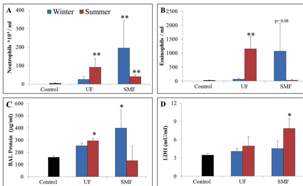
Fig. 3. Pulmonary response to summer and winter regional background PM. (A) Neutrophils, (B) Eosinophils, (C) BALF protein, and (D) LDH, expressed as mean \pm SEM, recovered in BALF 24 h post-exposure to 50 \mu\text{g} winter (blue) or summer (red) UF or SMF highly processed regional background PM. Asterisks (* p < 0.05 ; ** p < 0.0001 ) indicate significant differences from control (black bar). (For interpretation of the references to color in this figure legend, the reader is referred to the web version of this article.)
