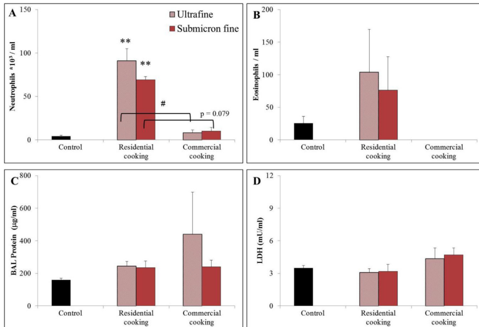
Fig. 7. Pulmonary response to summer residential and commercial cooking emissions. (A) Neutrophils, (B) Eosinophils, (C) BALF protein, and (D) LDH, expressed as mean \pm SEM, recovered in BALF 24 h post-exposure to 50 \mu g summer UF (light red) or SMF (dark red) residential and commercial cooking PM. Asterisks (* p < 0.05 ; ** p < 0.0001 ) indicate significant differences from control (black bar); # indicates significantly different from the SMF fraction as indicated by brackets. (For interpretation of the references to color in this figure legend, the reader is referred to the web version of this article.)
