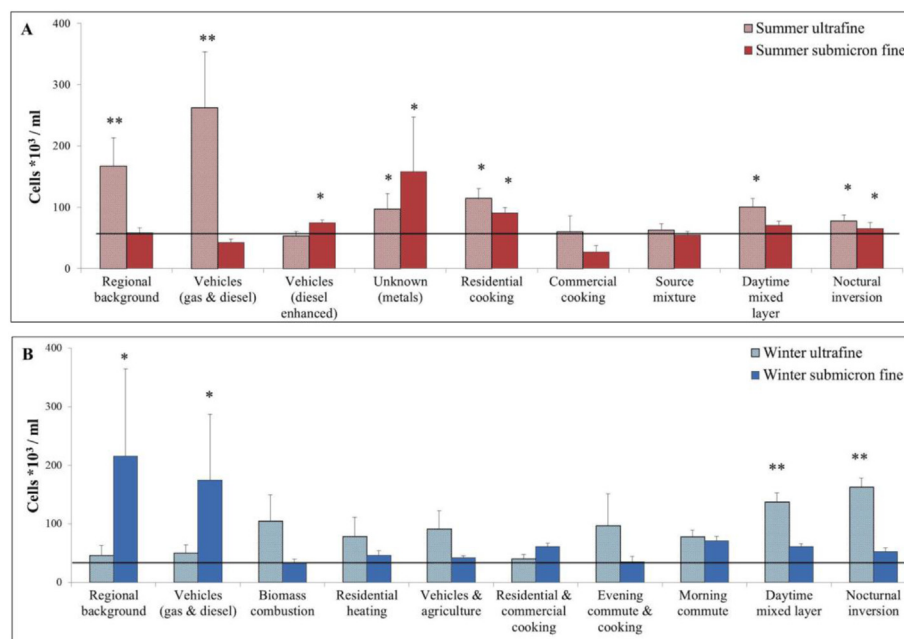
Fig. 1. Total pulmonary cells recovered in BALF 24 h post-exposure to 50 µg summer (A) or winter (B) UF (light shade) or SMF (dark shade) source-oriented PM. Asterisks (* p < 0.05 ; ** p < 0.0001 ) indicate significant differences from control (solid line). Data expressed as mean \pm SEM.
