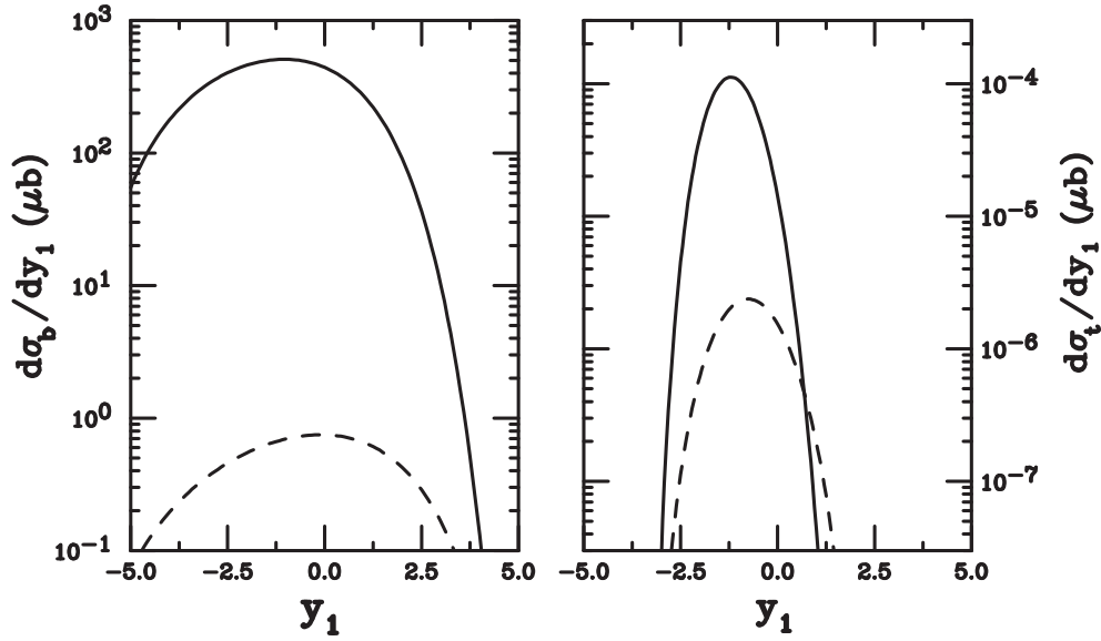
Figure 6: Rapidity distributions of bottom (left) and top (right) quarks produced in photonuclear collisions at the LHC. The solid and dashed curves are for Pb+Pb and O+O interactions, respectively. Here, the photon is emitted by the nucleus with positive rapidity; the complete cross section is the sum of this curve plus its mirror image. Shadowing is included using the parameterizations of Reference [62]. Adapted from References [89] and [90].
