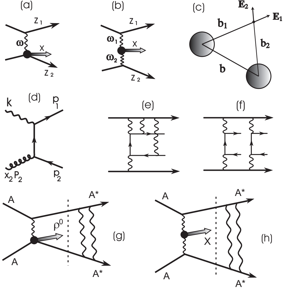
Figure 1: (a) One-photon and (b) two-photon processes in heavy ion collisions. (c) Geometrical representation of the photon fluxes at a point outside nuclei 1 and 2, in a collision with impact parameter b . The electric field of the photons at that point are also shown. (d) Feynman diagram for q\bar{q} production through photon-gluon fusion to leading order. (e,f) Example of higher order corrections to pair-production: (e) Coulomb distortion, and (f) production of multiple pairs. (g) The dominant diagram for Au + Au \rightarrow Au^* + Au^* + \rho^0 and (h) for Au + Au \rightarrow Au^* + Au^* + e^+e^- or a meson X . The dotted lines in panels (g) and (h) show how the mutual Coulomb nuclear excitation factorizes from the particle production.
