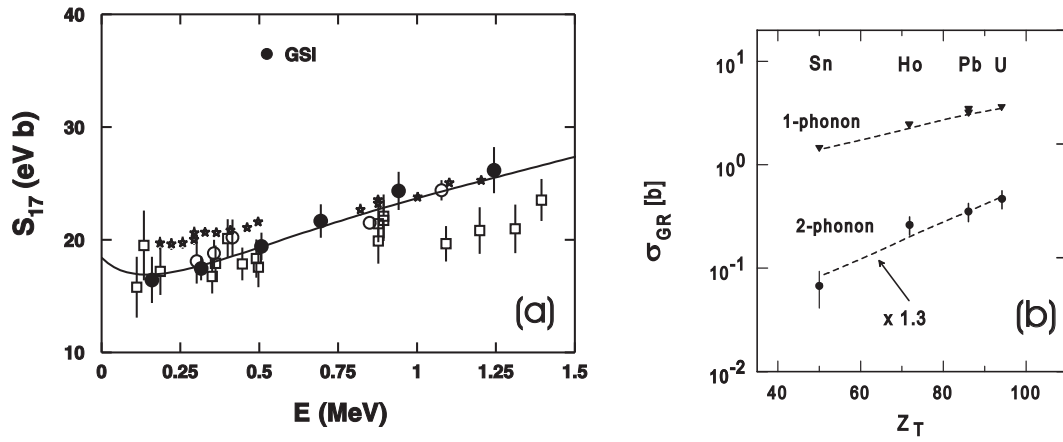
Figure 2: (a) S-factors ( S_{17} ) for the {}^7\text{Be}(p,\gamma){}^8\text{B} reaction. The GSI data was obtained using the Coulomb dissociation method [38]. The other data are from direct capture measurements [39]. (b) Cross sections for the excitation of the GDR (1-phonon) and the DGDR (2-phonon) in {}^{208}\text{Pb} projectiles incident on different targets. The dashed curves are theoretical calculations.
