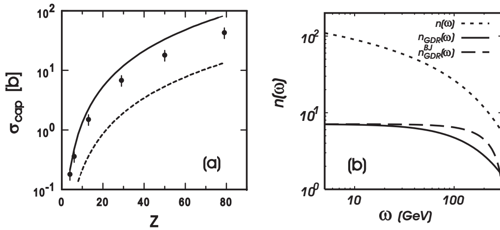
Figure 7: (a) Pair production with capture for \text{Pb}^{82+} (33 TeV) beams on several targets. The solid and dashed curves are theoretical calculations [152]. See text for more details. (b) The tagged total photon flux (accompanied by a single giant dipole resonance excitation) for a complete calculation (solid line) and a simplified 'box' integration (dashed line), compared to the untagged flux (dotted line), for gold at RHIC. Although tagging reduces the low-energy flux by an order of magnitude, at high energies, the difference is much smaller. From Reference [22].
