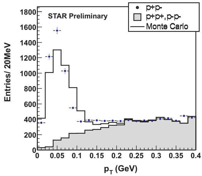
Figure 8: Transverse momentum distribution for events with exactly 2 reconstructed charged pions. Data from the STAR collaboration [74]. The Monte Carlo calculation is based on [75].
