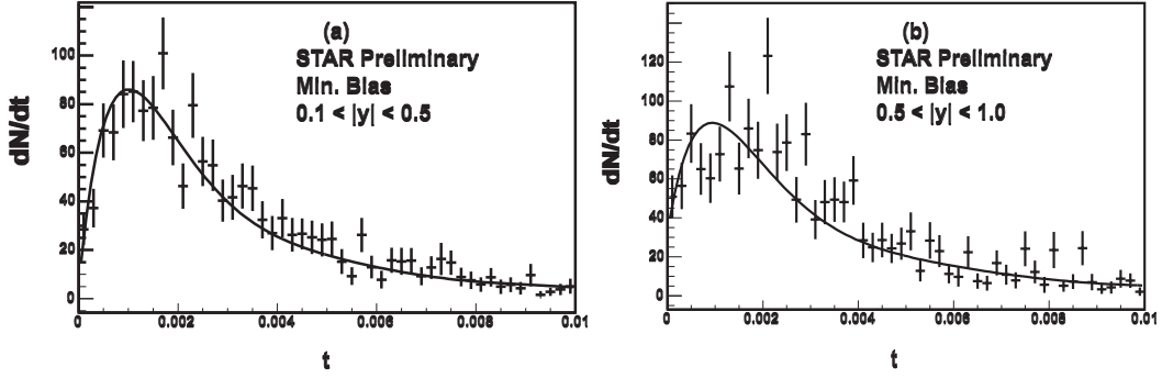
Figure 5: Efficiency corrected t_{\perp} spectrum for \rho^0 production in Au+Au collisions at RHIC with Coulomb breakup. The points are the data, and the solid curve is a fit to Equation 23. Interference causes the dip at low t \leq 0.001 (GeV/c)^2 [85].
