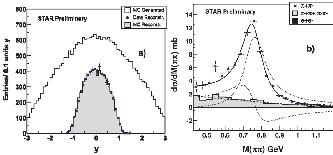
Figure 3: Rapidity (a) and invariant mass (b) distributions for coherent \rho^0 production in Au+Au interactions accompanied by mutual Coulomb breakup at \sqrt{s} = 200 A GeV, by the STAR collaboration. The dashed curves in b) corresponds to a relativistic Breit-Wigner function and a Söding interference term; the solid curve is the sum of the two. The dash-dotted curve describes the background from incoherent interactions [74].
