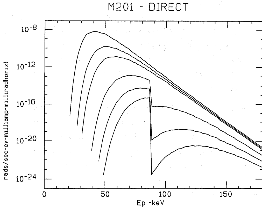
Figure 9: Direct beam dose spectra at beamline 5.02 MONO201 monochromator tank. The top three curves are for 2, 4 and 6 mm of steel, respectively. The bottom three curves are for a composite of 6 mm steel followed by 1, 2 and 3 mm of lead.
