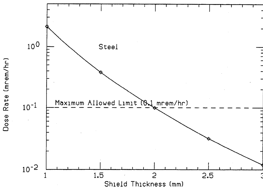
Figure 4: ALS \mu Probe hutch indirect (scattered) shield requirements.
