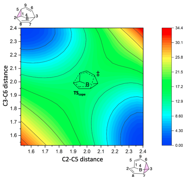
Fig. 10 2D potential energy surface for [3s,3s] sigmatropic shift of C_9H_9 .
