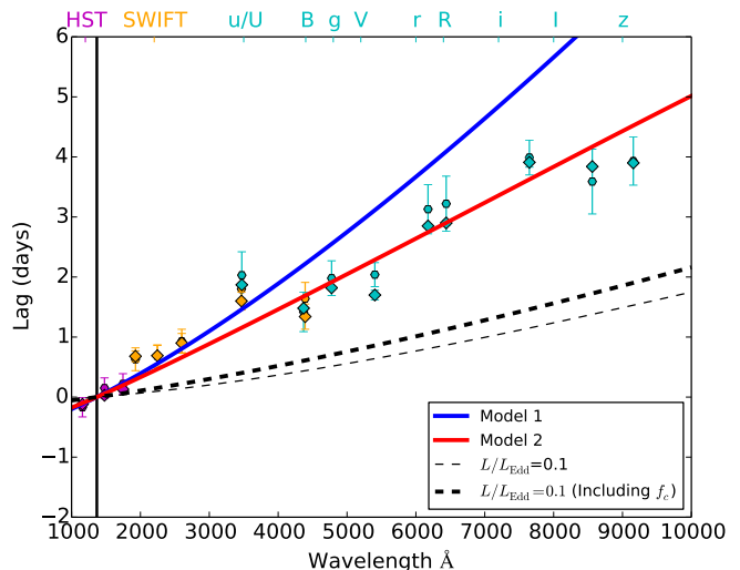
FIG. 7.— Mean lags with \alpha \equiv 0.75 (Model 1, blue) and \alpha fitted (Model 2, red). Markers show (circles) Javelin and (diamonds) CCF lags from Papers II and III for comparison. HST , Swift and ground-based observation are coloured by magenta, orange and cyan, respectively. Lags are plotted relative to the HST 1367 Å light curve (vertical black line). The thin dashed line shows the lag spectrum for a standard thin disk with L/L_{\text{Edd}} = 0.1 . Thick dashed lines show the lag spectrum for a standard thin disk with L/L_{\text{Edd}} = 0.1 that incorporates the partially covered blackbody model (Section 4).
