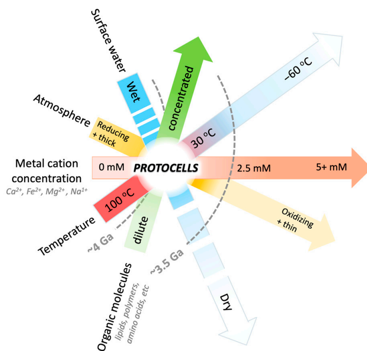
Figure 2. Uorable Mars? Schematic representation of the atmospheric, hydrological, and geochemical conditions that would have favored protocell formation on early Mars (‘orable’ conditions). Each bar represents a range of environmental conditions. Combined space where bars overlap represent conditions under which protocells can form. White lines on the surface-water bar indicate cycles of hydrated and dehydrated conditions, including short-term (hours, days, or weeks) and long-term (years, thousands of years, or millions of years) cycling in times of episodic surface water on Mars. Mars is speculated to have been a favorable environment for protocell formation ~4 Ga [1], then shifted out of such orable conditions ~3.5 Ga (gray dashed line) when a drying event resulted in the loss of the atmosphere and surface water. From that time forward, the evolution from protocells to living cells would have been more challenging. Uorability graph adapted from [1].
