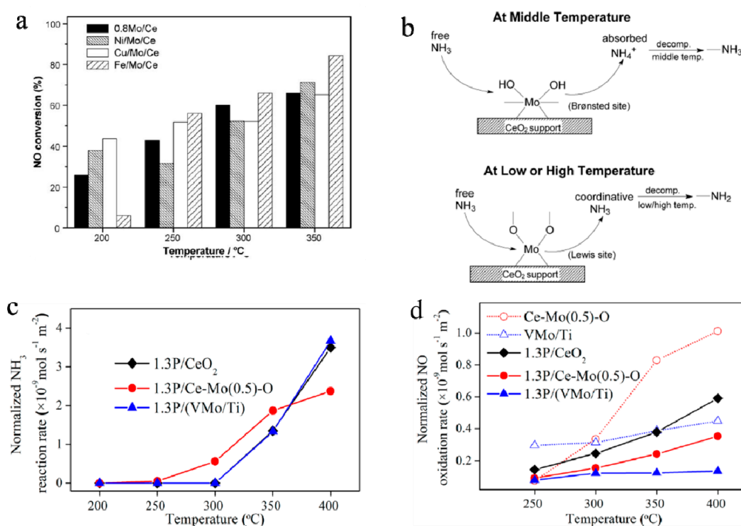
Figure 9. (a) The NO conversion for different catalysts in “ \text{NO} + \text{NH}_3 + \text{O}_2 ” reaction. (b) Schematic drawing of ammonia adsorption and decomposition on Brønsted and Lewis acid sites [116]. Reprinted with permission from [116]. Copyright 2009 Elsevier B.V. (c) \text{NH}_3 reaction rate vs. temperature over the Ce–Mo(0.5)–O and \text{CeO}_2 catalysts with different phosphorus content in \text{NH}_3 oxidation reaction. (d) Normalized NO oxidation rate vs. temperature in NO oxidation reaction over different catalysts after P poisoning [115]. Reprinted with permission from [115]. Copyright 2013 American Chemical Society.
