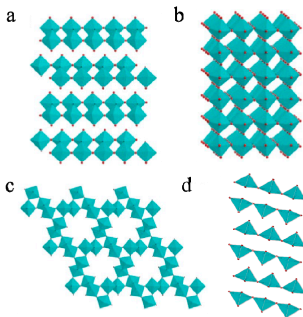
Figure 1. Atomic structures of different crystalline phases of \text{MoO}_3 . (a) \alpha - \text{MoO}_3 , (b) \beta - \text{MoO}_3 , (c) h- \text{MoO}_3 , and (d) \text{MoO}_3 -II. Reprinted with permission from [6]. Copyright 2018 American Chemical Society.
