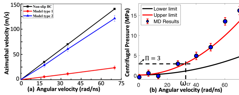
Figure 6. (a) Averaged azimuthal velocities of fluid near r = R_i as a function of angular velocity \omega for Model I and Model II. The curve “Non-slip BC” means v_\theta = R_i\omega . (b) Lower and Upper limits of the centrifugal pressure P_\omega derived from fluid dynamics and that obtained from MD calculations.
