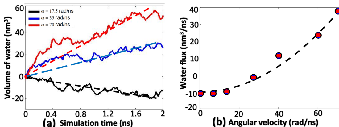
Figure 8. (a) Volume of filtrated water as a function of simulation time. (b) Water flux as a function of angular velocity.
