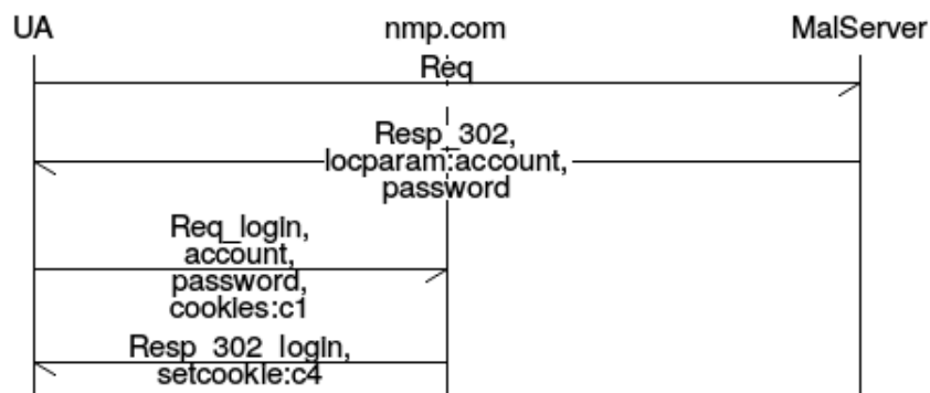
Figure 3.10: The session fixation attack for NeedMyPassword.com
