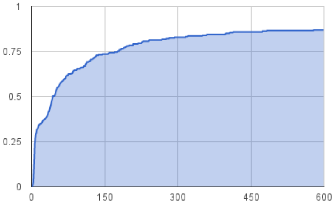
Figure 2.8: CDF of abstraction time (in seconds).
