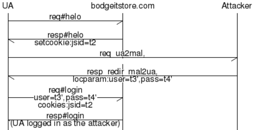
Figure 3.7: The message sequence chart for a login CSRF attack on the Bodgeit Store.
