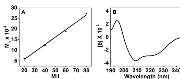
Figure 1. Synthesis and properties of poly(L-homoallylglycine), G^{HA} . (A) Number average molecular weight ( M_n ) of G^{HA} plotted as a function of monomer to initiator ratio (M:I) at complete monomer conversion using \text{Co}(\text{PMe}_3)_4 in THF ( r^2 = 0.9874 ). M_n values were determined by ^1\text{H} NMR analysis of PEG end-capped polymers. (B) Circular dichroism spectrum of G^{HA} in 15:1:2 cyclohexane:MeCN:IPA (0.5 mg/mL) at 20 °C. Molar ellipticity reported in \text{deg}\cdot\text{cm}^2/\text{dmol} .
