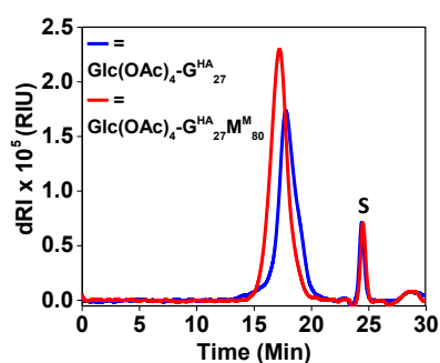
Figure 2. GPC Chromatograms of derivatized homo and diblock polypeptides Glc(OAc) 4 -G HA 27 (blue) and Glc(OAc) 4 -G HA 27 M M 80 (red) in HFIP containing 0.5 % (w/w) KTFa. S = solvent. RIU = arbitrary refractive index units.
