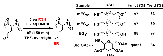
Figure 3. Thiol-ene modification of G HA (4 mg/mL) in THF with UV irradiation followed by overnight stirring at ambient temperature. Funct = percentage of side-chain modification. Yield = total isolated yield of purified polypeptide. quant. = quantitative
