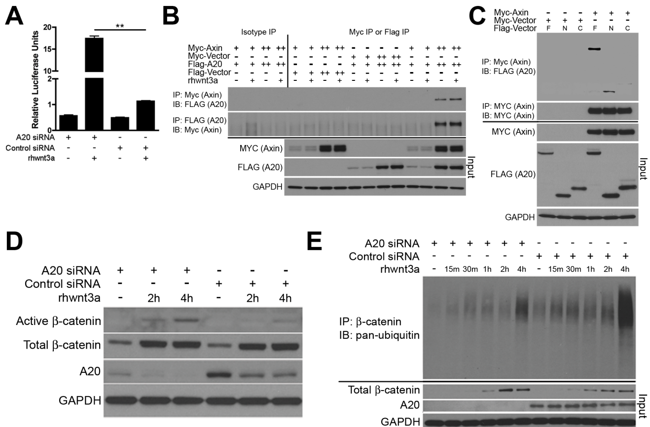
Figure 3. A20 supports \beta -catenin ubiquitination and degradation through an interaction with the destruction box. (A) Luciferase assay showing transcriptional activity of a \beta -catenin dependent TCF/LEF4 reporter in RKO cells. Cells were treated with A20 specific or control siRNA and recombinant human wnt3a (rhwnt3a) as indicated. Relative luciferase units (RLU) are shown. **indicates p < 0.01 . (B) Co-precipitation of A20 with Axin. RKO cells transfected with the indicated expression plasmids were lysed, immunoprecipitated (IP) for the indicated epitope tag, and immunoblotted (IB) for the indicated proteins. Cells were stimulated with rhwnt3a or control as indicated for four hours. Input levels of MYC, FLAG, and GAPDH are shown as controls below. (C) Co-precipitation of partial A20 proteins with Axin. Co-transfection experiments as in (B). Input levels of MYC, FLAG, and GAPDH shown below. (D) A20 suppresses wnt3a stimulated induction of \beta -catenin expression. Immunoblot analyses of active and total \beta -catenin expression in RKO cells treated with A20 specific or control siRNA. A20 and GAPDH levels shown below as loading control. (E) A20 supports wnt3a stimulated \beta -catenin ubiquitination. RKO cells were treated with A20 specific or control siRNAs and wnt3a for the indicated times. Lysates were immunoprecipitated for \beta -catenin followed by immunoblotting for ubiquitin. Input amounts of beta-catenin, A20, and GAPDH proteins shown below as controls. All data are representative of three or more independent experiments. doi:10.1371/journal.pone.0062223.g003
