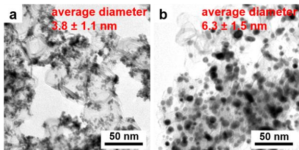
Supplementary Fig. 6 | TEM images of commercial Pt/C catalyst. a, before MEA test. b, after 30k square wave cycles in the MEA test.
