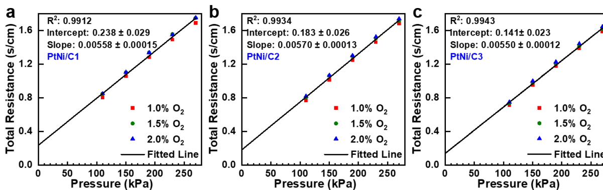
Supplementary Fig. 10 | The measured total oxygen transport resistances in MEAs plotted with the total pressure during the measurement. a , PtNi/C1, b , PtNi/C2, c , PtNi/C3. The total oxygen transport resistance can be separated into pressure dependent part ( R^{P-d} ) and pressure independent part ( R^{P-ind} ), which represents the Knudsen diffusion and diffusion of oxygen through the ionomer layer in the catalyst layer 50,51 . Thus, the pressure independent part is critical for oxygen transport in an operating fuel cell. The relationship of total oxygen resistance ( R_{total} ), pressure dependent part of oxygen transport resistance ( R^{P-d} ), and pressure independent part of oxygen transport resistance ( R^{P-ind} ) can be expressed in the following Eq. S1 (noted in the Method part “Oxygen Transport Resistance Test for MEA”).
