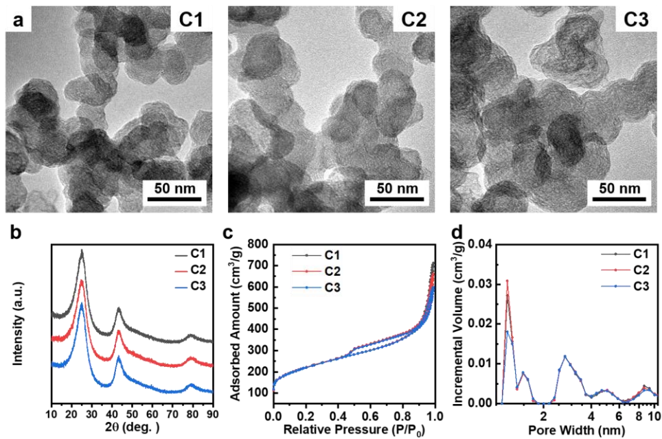
Supplementary Fig. 2| Characterization of carbon materials. a , TEM images. b , XRD spectra. c , N_2 adsorption-desorption isothermal plots. d , pore size distribution calculated from density function theory (DFT) model using nitrogen isothermal plots in c .
