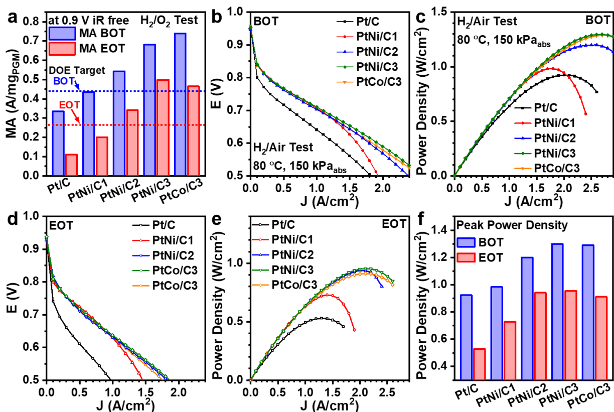
Fig. 2| Membrane electrode assembly (MEA) test. a , Comparison of mass activities obtained in the H 2 /O 2 test at the beginning of test (BOT; before ADT) and end of test (EOT; after ADT). b-e , H 2 /Air test. b , polarization plots at BOT. c , power densities plots at BOT. d , polarization plots at EOT. e , power densities plots at EOT. f , Comparison of peak power densities. The MEA test was performed at 80 °C and 150 kPa abs pressure unless specifically noted.
