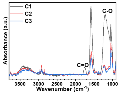
Supplementary Fig. 1 | ATR-FTIR spectra of our three carbon materials with surface oxygens.
