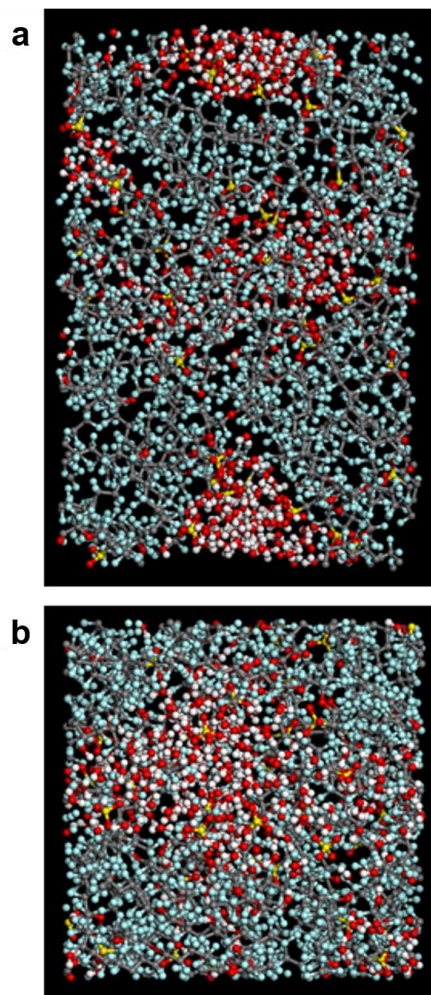
Supplementary Fig. 9| Predicted structures from ReaxFF MD. The Hydrated PFSA ionomer structure contains non-polar hydrophobic parts (polytetrafluoroethylene [PTFE] backbone) and hydrophilic sulfonic acid ( -\text{SO}_3^- ) parts. a , The side view of PFSA ionomer molecules with a cluster of waters ( 12 \text{ H}_2\text{O}/-\text{SO}_3^- ) at the carbon ionomer interface. b , The top view of the panel a . The structures were equilibrated at 600 K for 200 ps and cooled down to 300 K at 0.2 fs time step (gray: carbon; light cyan: Fluorine; red: oxygen; white: hydrogen; yellow: sulfur).
