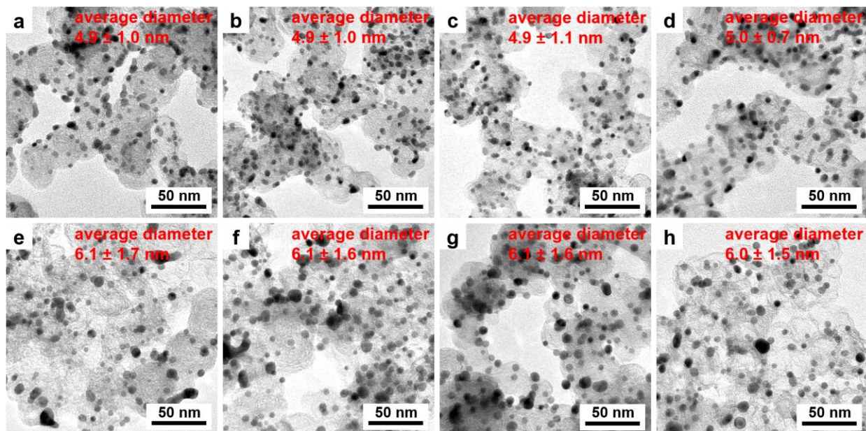
Supplementary Fig. 3| TEM images of catalysts. Catalysts before MEA test a , PtNi/C1, b , PtNi/C2, c , PtNi/C3, d , PtCo/C3. Catalysts after 30k square wave cycles in MEA test e , PtNi/C1, f , PtNi/C2, g , PtNi/C3, h , PtCo/C3.
