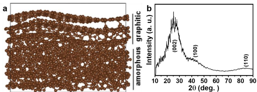
Supplementary Fig. 7| Predicted Core-shell like carbon substrate structure with its predicted XRD pattern. a , The predicted carbon substrate has a structure similar to that obtained by experimentally. It consists of three layers of graphitic carbon on top of amorphous carbon on the bottom. We heated the amorphous carbon to 6000 K and quenched to 300 K, followed by heating to 3500 K temperature followed by quenching at 300 K at 100 K/ps rate. The final carbon density in our structure is 2.15 g/cm 3 . b , The predicted X-ray diffraction pattern (XRD), which is similar to experimental data as shown in Supplementary Fig. 2b . The XRD used Cu source radiation with powder diffraction technique at 0.05 step size.
