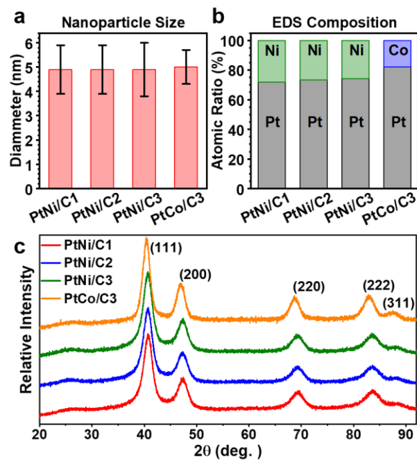
Supplementary Fig. 4| Characterization of prepared catalysts. a , The diameter of nanoparticles based on TEM images in Supplementary Fig. 3. b , EDS composition. c , XRD spectra of prepared catalysts.
