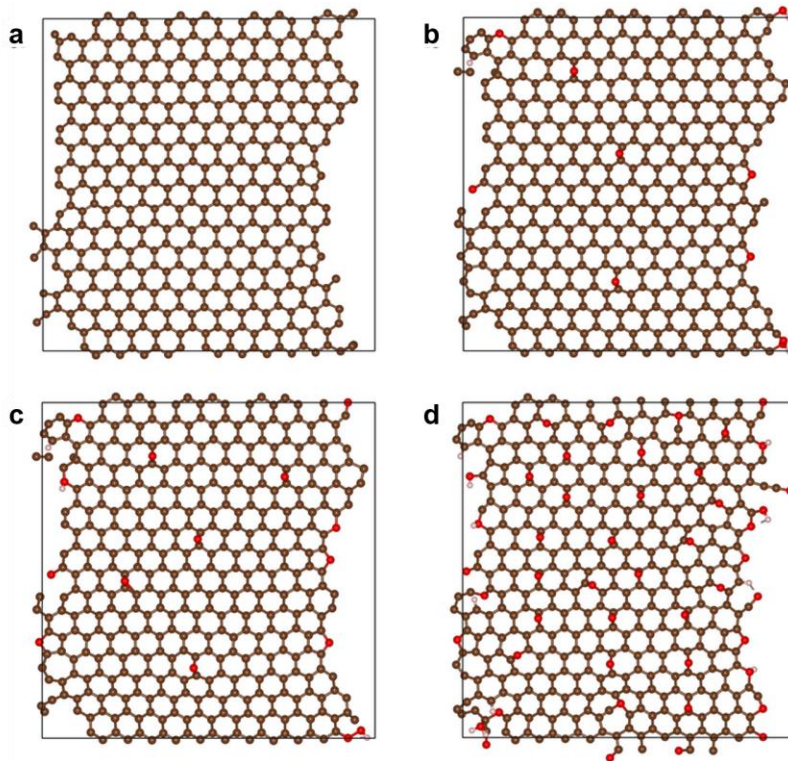
Supplementary Fig. 8| The carbon surface oxidation patterns used in the MD simulations. a , pure graphitic surface (0% oxygen). b , c , and d are 2.5%, 4.0% and 12.0% oxygen to carbon ratios. All structures were minimized and equilibrated for 100 ps at 300K temperature and 0.2 fs time step. (coffee: carbon, red: oxygen, off-white: hydrogen).
