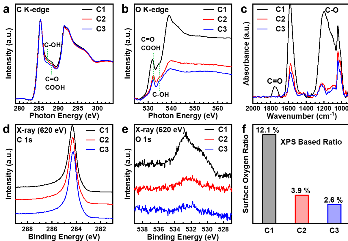
Fig. 1| Characterization of carbon materials. a, b, synchrotron-based NEXAFS spectra for carbon K-edge (a) and for oxygen K-edge (b). The intensity is normalized by sample loading. c, ATR-FTIR spectra. d, e, synchrotron-based XPS spectra for carbon 1s (d) and oxygen O 1s (e). f, the surface oxygen ratio for three carbon samples evaluated; C1, C2, and C3.
