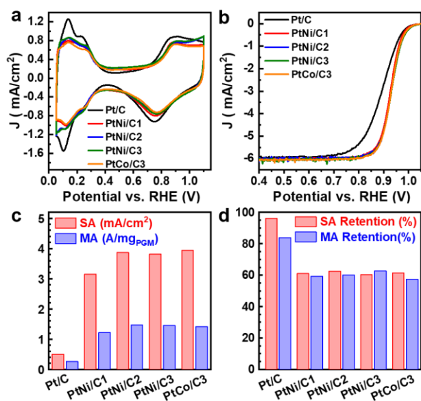
Supplementary Fig. 5 | Rotating disk electrode (RDE) test of catalysts. a , cyclic voltammograms of tested in N 2 saturated 0.1 M HClO 4 . b , ORR polarization curves in O 2 saturated 0.1 M HClO 4 (1600 rpm). c , comparison mass activities (MA) and specific activities (SA) d , comparison of retention ratios of mass activities.
