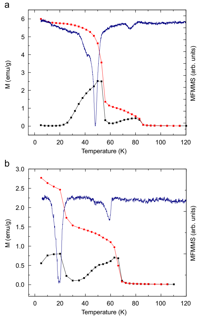
Fig. 6. ZFC (—■—) and FC (—●—) magnetization curves at 100 Oe; microwave absorption response as a function of temperature (solid blue line) for samples (a) \text{Pr}_5\text{Si}_3\text{C}_{1.5} and (b) \text{Pr}_5\text{Si}_3\text{C}_3 . (For interpretation of the references to color in this figure legend, the reader is referred to the web version of this article.)
