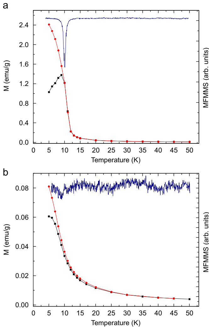
Fig. 2. ZFC (—■—) and FC (—●—) magnetization curves at 100 Oe; microwave absorption response as a function of temperature (solid blue line) for samples (a) Pr 5 Si 3 and (b) Pr 3 Si 2 (intended composition). (For interpretation of the references to color in this figure legend, the reader is referred to the web version of this article.)
