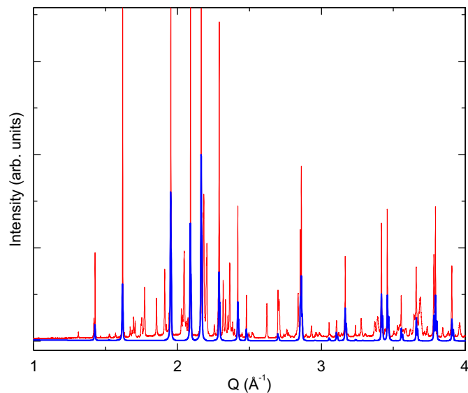
Fig. 7. X-ray diffraction patterns for sample \text{Pr}_5\text{Si}_3\text{C}_3 (thin red lines). Simulated X-ray diffraction pattern for phase \text{Pr}_3\text{Si}_2\text{C}_2 (thick blue lines). (For interpretation of the references to color in this figure legend, the reader is referred to the web version of this article.)
