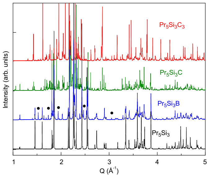
Fig. 5. HRXRD patterns for samples undoped \text{Pr}_5\text{Si}_3 (bottom black), \text{Pr}_5\text{Si}_3\text{B} (third to the top blue), \text{Pr}_5\text{Si}_3\text{C} (second to the top green) and \text{Pr}_5\text{Si}_3\text{C}_3 (top red). Dots indicate the \text{PrB}_4 diffraction maxima. (For interpretation of the references to color in this figure legend, the reader is referred to the web version of this article.)
