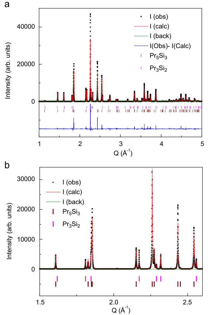
Fig. 3. (a) Rietveld refinement profile of the HRXRD data for the undoped sample. Tick marks indicate reflections coming from the Pr 5 Si 3 and Pr 3 Si 2 phases. (b) Zoom of (a).
