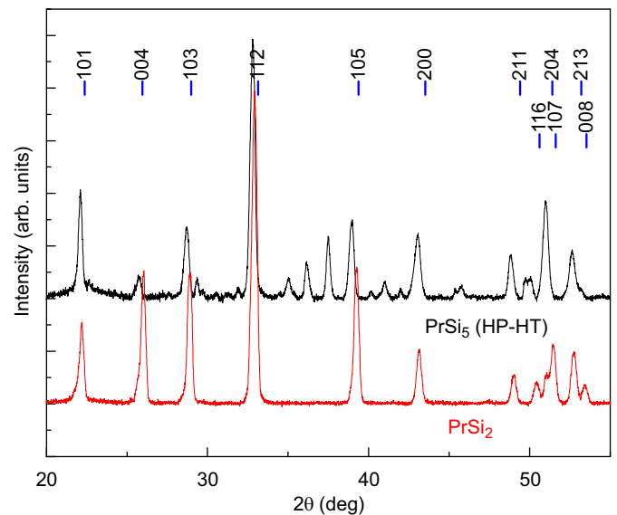
Fig. 1. X-ray diffraction patterns for: (bottom red) starting material \text{PrSi}_2 ; (top black) intended composition \text{PrSi}_5 after HP–HT synthesis. Tick marks indicate reflections coming from the \text{PrSi}_2 phase. (For interpretation of the references to color in this figure legend, the reader is referred to the web version of this article.)
