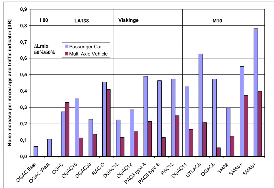
Figure 4.4. \Delta L_{\text{Mix}50/50} noise level increase per Mixed Indicator as the change of noise predicted as a combination of physical age and traffic load where the age counts for 50 % and the traffic load counts for 50 %.
