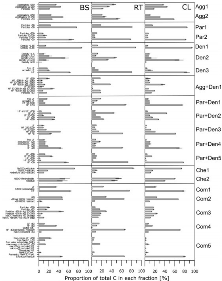
Fig. 2. Average proportion of total carbon (C) in each fraction for the Braunschweig (BS), Rotthalmünster (RT), and Le Closieux (CL) soils, depending on the method used (for explanation of ID codes, see Table 2) with standard error (bars). LF = light fraction; HF = heavy fraction; agg = aggregates; rem. = remaining; ext = extractable. Units in the fraction descriptions are \mu\text{m} , or \text{g cm}^{-3} in the case of density fractions.
