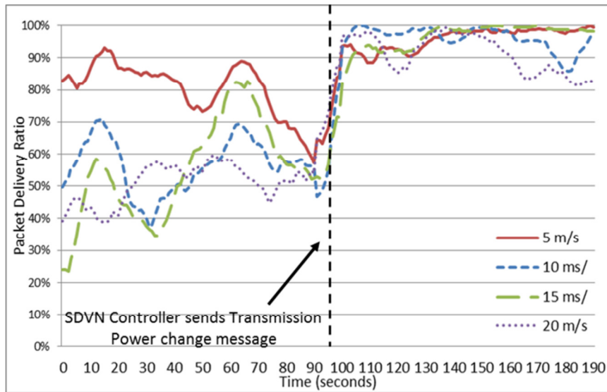
Figure 4.18 SDVN controlling Transmission Power and Range
