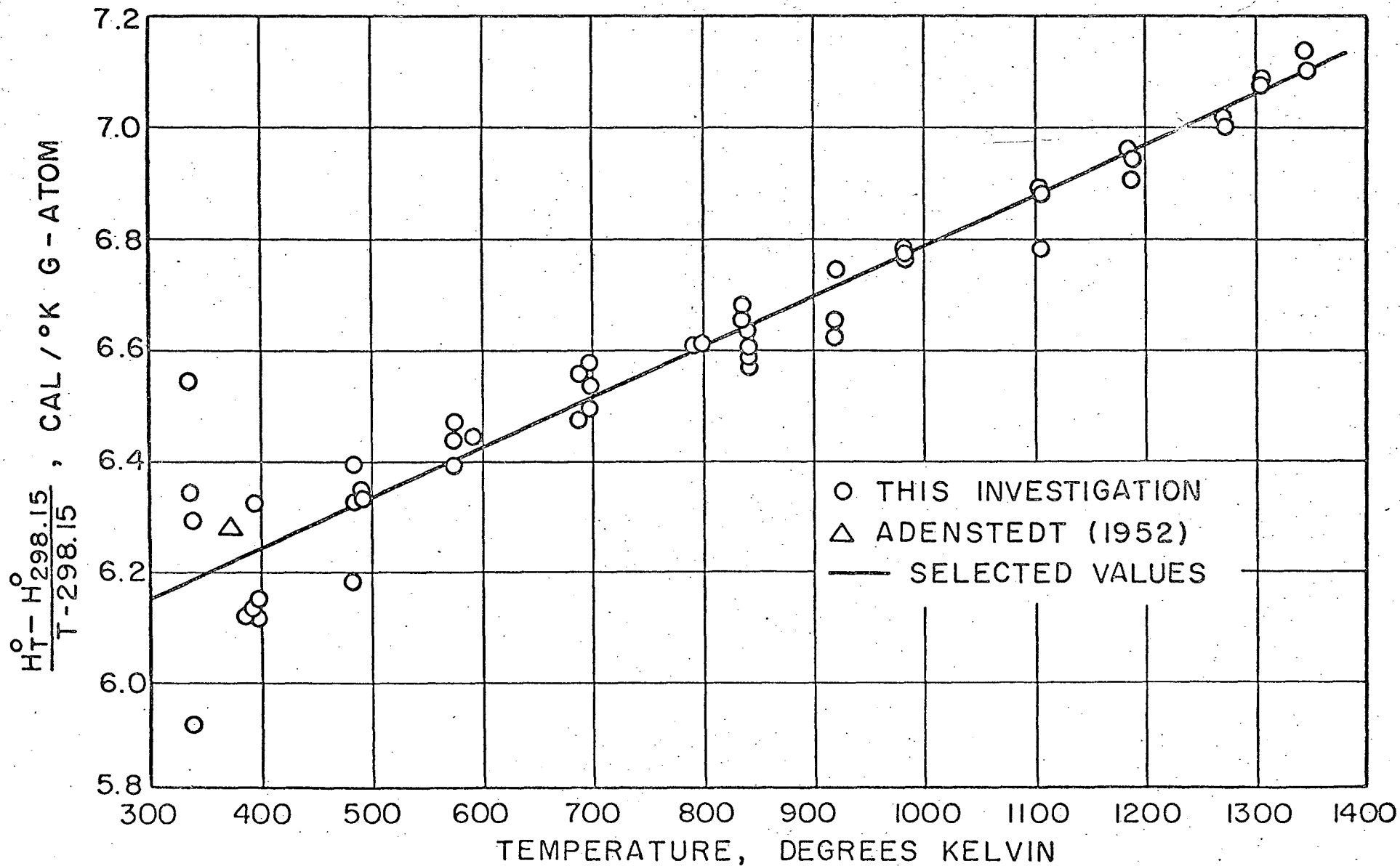
Figure 1. Heat content of hafnium expressed in terms of the function \frac{(H_T^0 - H_{298.15}^0)}{(T - 298.15)} .
