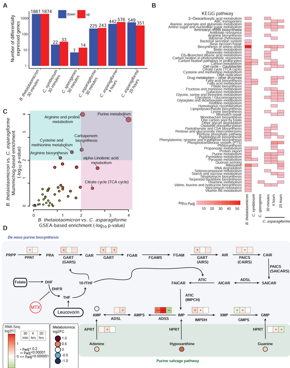
Figure 3. Impact of MTX on human gut bacterial transcriptomes and metabolomes. (A) A variable number of transcripts, as determined by RNA-seq, were differentially expressed ( p_{adj} < 0.2 , DESeq) upon 30 minutes of MTX 100 \mu\text{g/ml} (compared to vehicle control) in 4 bacterial isolates with varying sensitivity to the growth inhibitory effects of the drug ( n=3 per treatment). Clostridium asparagifforme was also treated for 4 and 20 hours. (B) A heatmap of KEGG pathway enrichments ( p_{adj} < 0.05 , BH corrected) of differentially expressed genes ( p_{adj} < 0.2 , DESeq) in bacterial isolates treated with 100 \mu\text{g/ml} of MTX vs. vehicle control ( n= 3 per treatment / isolate). Colors represent log 10 adjusted p-value. (C) Pathways enriched among metabolite features exhibiting a significant interaction between bacterial isolate and MTX treatment in the supernatants of B. theta and C. asparagifforme cultures exposed to MTX (100 \mu\text{g/ml} for 24 hours) as assessed by
