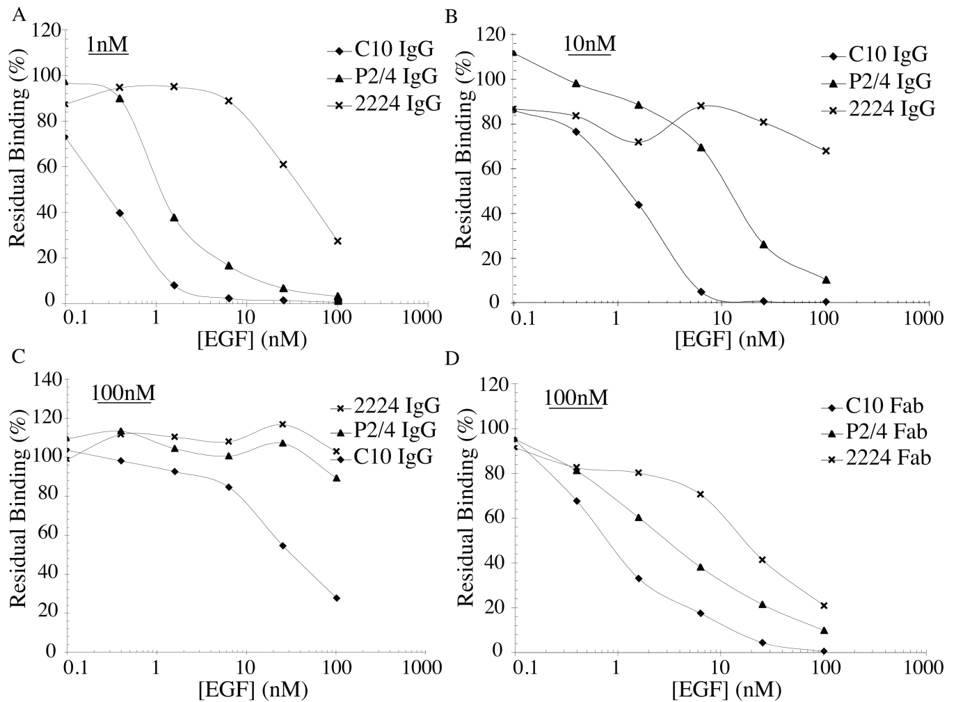
Figure 2. Impact of intrinsic and apparent antibody affinity and concentration on the ability of EGF to inhibit antibody binding to EGFR-overexpressing cells. A, at 1 nM IgG, EGF inhibited the binding of IgG in proportion to their intrinsic affinities; At 10 nM (B) and 100 nM (C) IgG concentration, there was less effect of EGF on IgG binding, especially of the higher intrinsic affinity 2224 and to a lesser extent P2/4. (D) EGF inhibited the binding of Fab in proportion to their intrinsic affinities. Comparing (C) to (D), it is clear that an increase in apparent affinity due to IgG avidity significantly reduces the reduction of antibody binding by EGF.
