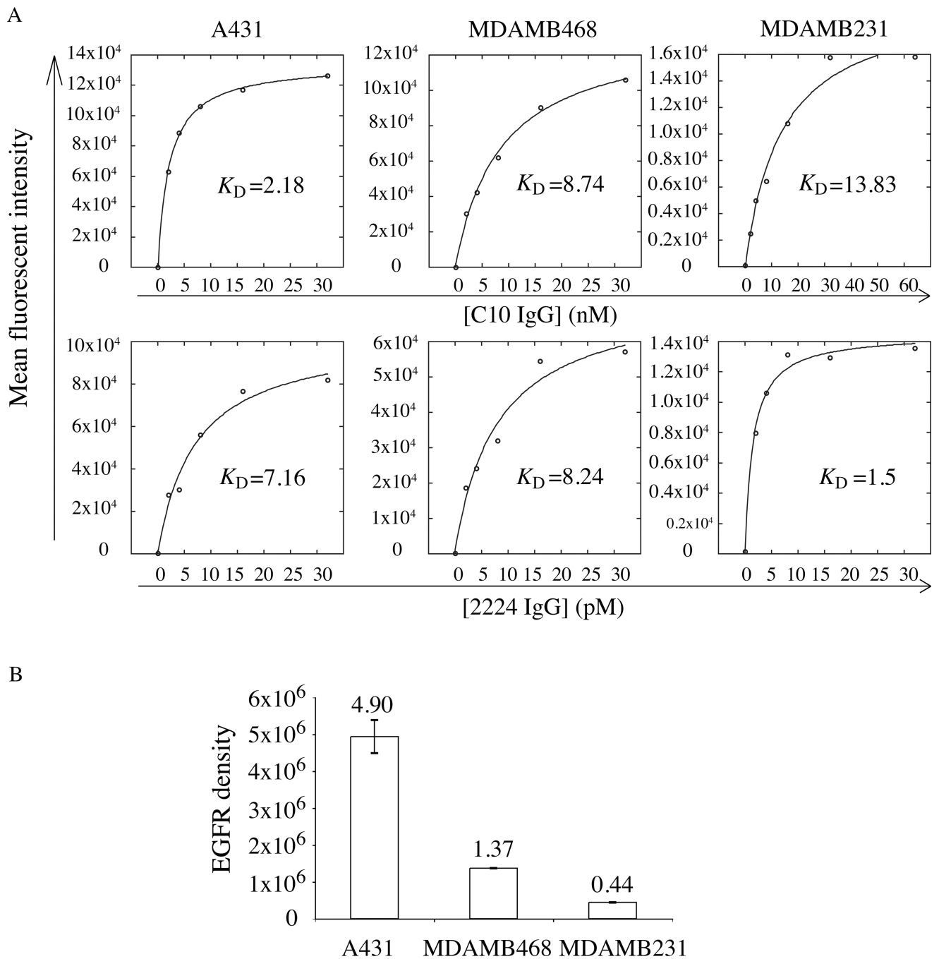
Figure 1. Impact of EGFR density on the apparent binding affinities of IgG to EGFR-overexpressing cells. A, low and high intrinsic affinity IgG (C10 and 2224) had their functional affinities measured on cells of varying EGFR density (B).
