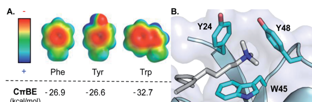
Fig. 1 (A) Electrostatic potential maps of Phe, Tyr, and Trp and the calculated cation- \pi binding energy ( C\pi BE ) of the aromatic side chain. Electrostatic potentials were calculated in Spartan at the B3LYP/6-31G* level of theory (+100 to -100 kcal mol -1 ). C\pi BE are based on gas phase interactions of the aromatic side chain with Na + . (B) Aromatic cage (cyan) of the HP1 chromodomain bound to Kme3 (silver). PDB ID: 1KNE.
