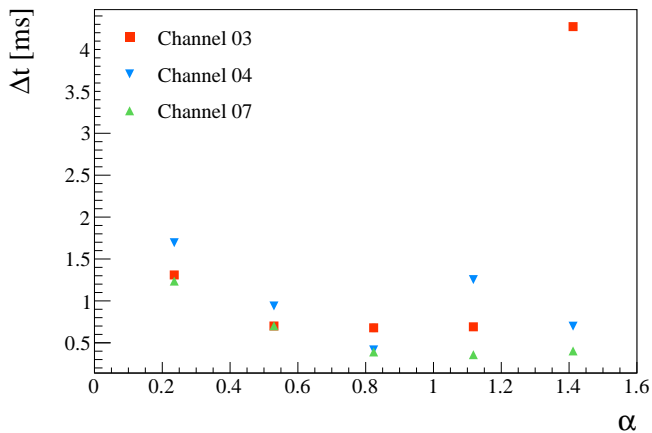
FIG. 6. \Delta t thresholds corresponding to \varepsilon_{\text{rej}} = 90\% for each configuration of \alpha obtained for the three channels. The two outliers at \alpha = 1.12 for Channel04 and \alpha = 1.41 for Channel03 are likely due to sub-optimal detector conditions while collecting data for \Delta t = 1 ms.
