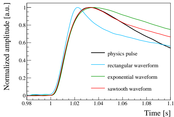
FIG. 1. Overlay of the rising edge and initial part of the decay for a particle pulse (black) and heater pulses excited by rectangular (blue), exponential (green) and sawtooth (red) waveforms.
