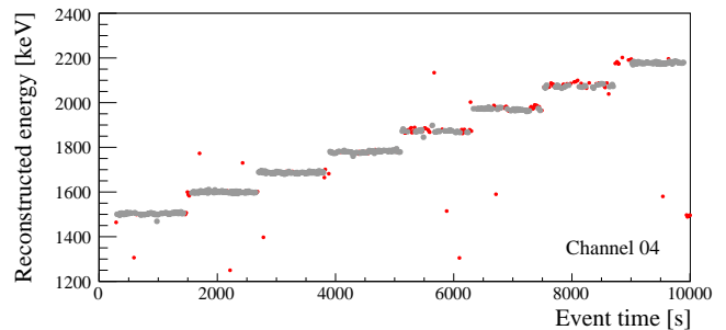
FIG. 3. Time distribution of the events in one of the pile-up runs. Each interval corresponds to a different \alpha/\Delta t configuration. In this sequence, \alpha is fixed to 0.24 while \Delta t goes from 1 ms to 11 ms (from left to right). The gray dots represent the events selected as heater pulses, the red dots the discarded ones; we keep only clean events with a single trigger fired in the 5-s window.
