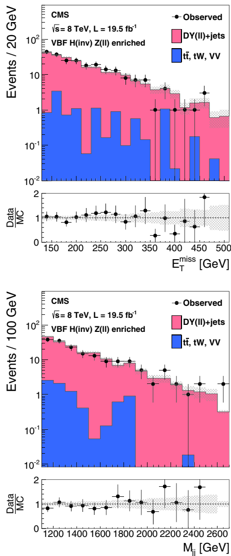
Fig. 3 The E_T^{\text{miss}} (top) and M_{ij} (bottom) distributions in the relaxed Z control region of the VBF search, with no requirements on \Delta\eta_{ij} , \Delta\phi_{ij} , or CJV, and with the M_{ij} requirement relaxed to 1,000 GeV. The simulated background from different processes is shown cumulatively, and normalized to the data, with its systematic uncertainty shown as a hatched region. The lower panels show the ratio of data to the simulated background, again with the systematic uncertainty shown as a hatched region
