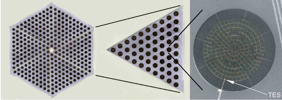
Figure 3. Left panel: Montage image of a photograph of a single real TES “wedge” of spider bolometers replicated electronically to show how a final array will look. Each wedge is designed to be identical and has 55 bolometers. The entire array will have 330 bolometers and be 17 cm in diameter. Center panel: Photograph of wedge of 55 spider web TES bolometers. Wedge is 8 cm on a side. Suspended spider web absorbers are fabricated from 1\ \mu\text{m} thick silicon nitride. The membrane is released from the front side using a gaseous xenon difluoride etch. Bolometers are 3.5 mm diameter with 0.5 mm long legs. Wiring layer is superconducting aluminum. This array was fabricated in the U.C. Berkeley microfabrication facility. Right panel: Close up of 55 element bolometer wedge. Sensors are an Al/Ti proximity effect sandwich TES, located at the edge of the membrane and electrically connected with superconducting leads.
