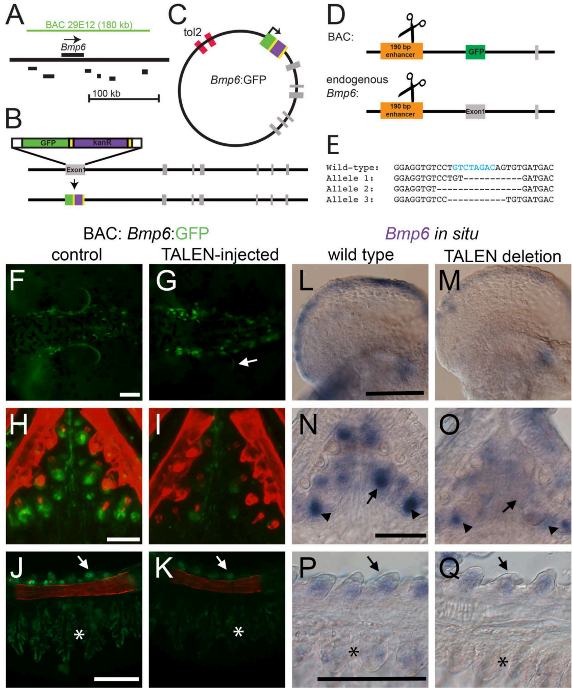
Fig. 6. The 5' 190 bp enhancer is necessary for Bmp6 expression (A) Schematic of the genomic location of the 180 kb CHORI BAC29E12 with respect to Bmp6 and nearby genes (coding regions shown in black are Ipo4 , Pdcd6 , Txndc5 , Muted , Eef1e1 , and Slc35b3 from left to right). (B) Recombineering strategy for introducing GFP into the first exon of Bmp6 ; grey bars indicate exons. (C) Final circular BAC with inverted Tol2 sites for transposition and GFP reporter (not to scale). (D) Strategy for introducing TALEN lesions into the 190 bp 5' enhancer. The same TALENs were used to target the enhancer in stable transgenic BAC fish and at the endogenous Bmp6 locus (diagram not to scale)
