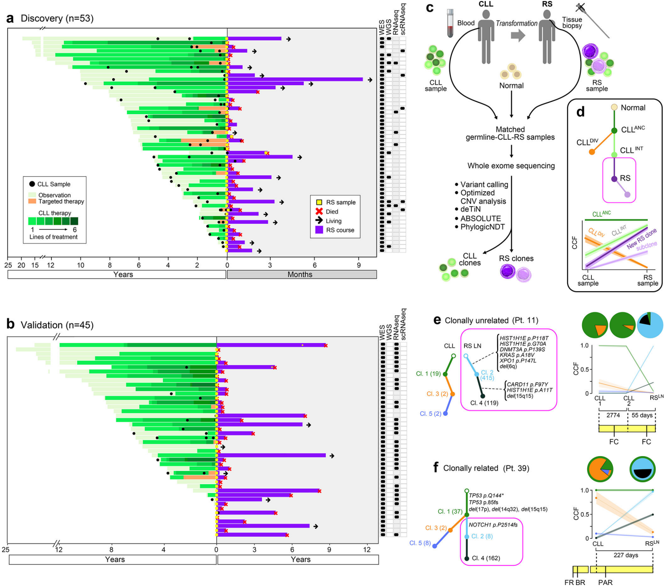
Fig. 1. Developing an analytic framework for detecting Richter Syndrome (RS)-specific clones. a , Disease course of 53 RS patients from CLL diagnosis in relationship to lines of therapy and sample collection. b , Disease course of 44 of 45 RS validation cohort patients from CLL diagnosis in relationship to lines of therapy and sample collection (1 patient with missing data). c , Computational schema for deciphering CLL and RS clones within RS biopsy samples. d , Inset shows labeled sample phylogenetic tree with associated sample cancer cell fraction (CCF) plot. Phylogenetic trees with CCF clustering, clonal abundance and associated patient disease course in representative clonally unrelated ( e ) and related ( f ) cases.
