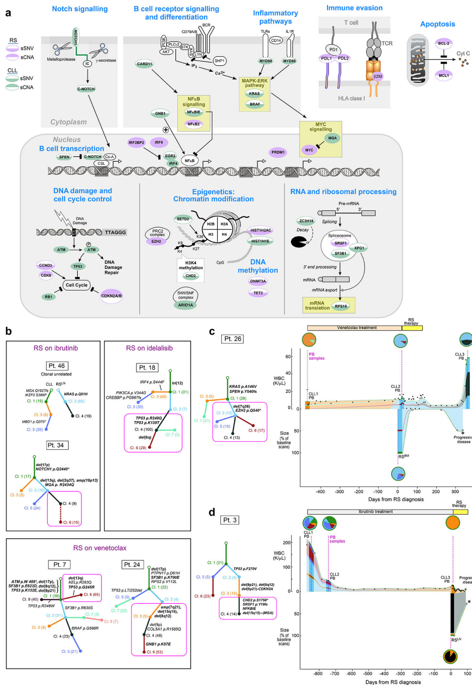
Fig. 3. Tracing evolution of RS on targeted agent therapy a , Pathways altered in CLL transformation to RS include CLL phase alterations (light green) and new drivers identified in RS (light purple). sSNV (top shading) and sCNA (bottom shading). b , Trees depicting clonal evolution of CLL to RS in seven select patients who developed RS on novel agents. Recurrent RS drivers indicated in bold. c-d , Evolution of RS from CLL showing clonal composition and absolute tumor burden over time based on serial sampling for two patients. Left panel - a phylogenetic tree with associated driver events. (Magenta square, RS clones). Right panel - relative abundance of CLL in peripheral
