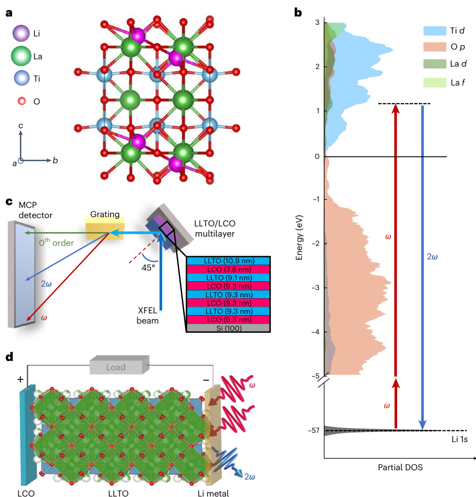
Fig. 1 | LLTO structure and experimental geometry. a , Basic crystal structure of LLTO, consisting of alternating Li-rich and -poor layers of Ti and O octahedra. b , Calculated partial density of states (DOS) for LLTO and indicated transitions for the XUV-SHG probe. c , Overview of the experimental setup used for measurement of XUV-SHG data in reflection geometry. The inset shows the
