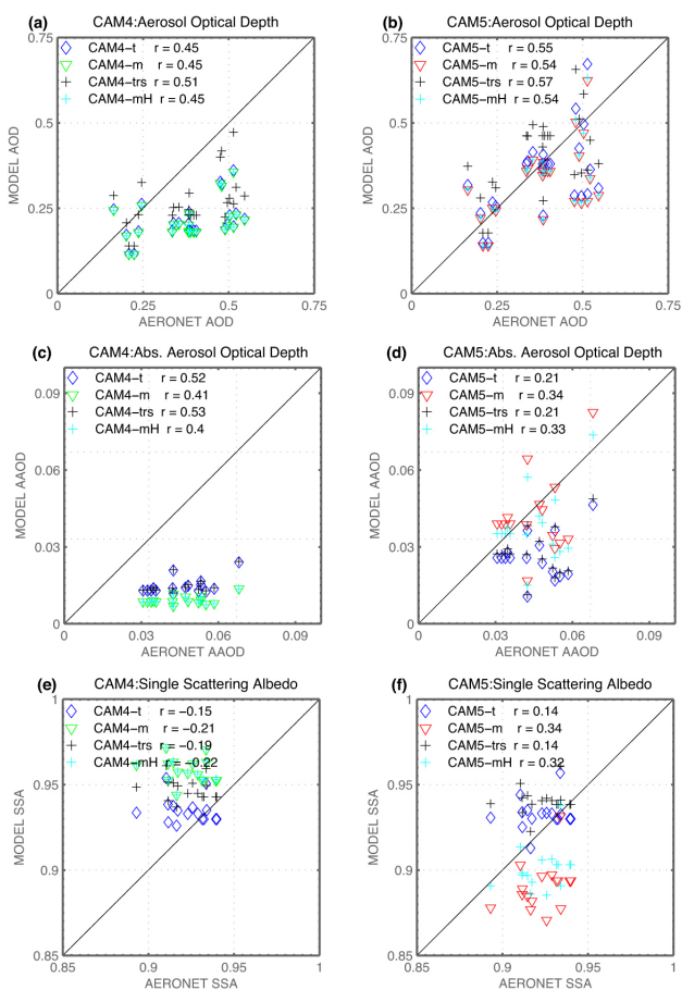
Figure 15. Annually averaged modeled aerosol optical depth (a, b), absorbing aerosol optical depth (c, d) and single scattering albedo (e, f) compared to annually averaged AERONET retrievals at 533 nm at sites where modeled AOD_{\text{dust}} > AOD_{\text{total}} \cdot 0.5 . CAM4 (a, c, e) and CAM5 (b, d, f) are shown for tuned dust, mineralogy, tuned dust + release size and mineralogy with hematite in soil clay only.
