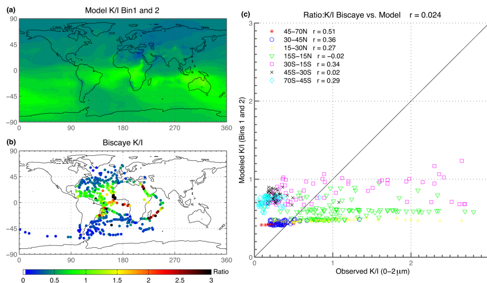
Figure 7. Kaolinite/illite mineral ratio of wet and dry deposition for bin 1 and bin 2 from CAM4 (a) (kg K / kg I) and from characteristic basal X-ray diffraction maxima ratios of K / I of ocean core sediments (b) (Biscaye, 1965). Data are segregated by latitude bands in scatterplot (c).
