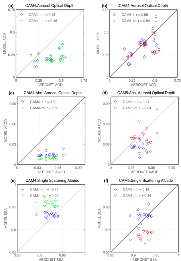
Figure 9. Annually averaged modeled aerosol optical depth (a, b), absorbing aerosol optical depth (c, d) and single scattering albedo (e, f) at 533 nm compared to annually averaged AERONET retrievals at sites where modeled AOD_{\text{dust}} > AOD_{\text{total}} \times 0.5 . CAM4 (a, c, e) and CAM5 (b, d, f) are shown.
