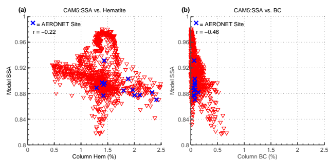
Figure 11. Model single scattering albedo from CAM5 with mineralogy is compared to total percent column hematite (a) and total percent column black carbon (b). The locations of AERONET sites used in the comparison in Fig. 9 are plotted in blue.
