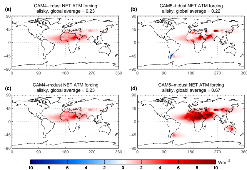
Figure 13. Spatial distribution of annual all-sky radiative forcing (SW + LW) in the atmosphere for CAM4 with tuned dust and with mineralogy (a, c) and for CAM5 with tuned dust and mineralogy (b, d).
