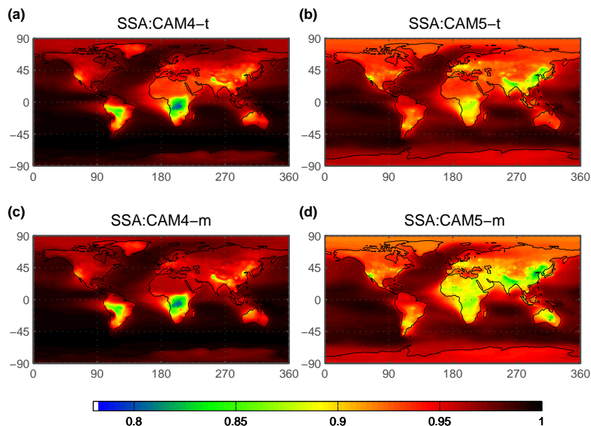
Figure 16. Model single scattering albedo for CAM4 with tuned dust (a), CAM5 with tuned dust (b), CAM4 with mineralogy (c) and CAM5 with mineralogy (d).
