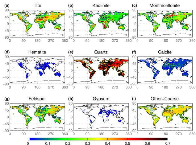
Figure 1. Mineral maps for CAM4 and AM5 based on work by Claquin et al. (1999) and Nicovic et al. (2011). Illite (a), kaolinite (b) and montmorillonite (c) are clay-sized ( 0\text{--}2\ \mu\text{m} ). Hematite (d) has the same distribution for both clay-sized and silt-sized ( 2\text{--}20\ \mu\text{m} ). Quartz (e), calcite (f), feldspar (g), gypsum (h) and other coarse (i) are silt-sized. CAM4 includes illite (a), kaolinite (b), montmorillonite (c), hematite (d), quartz (e), calcite (f), feldspar (g) and gypsum (h). CAM5 includes illite (a), kaolinite (b), montmorillonite (c), hematite (d) and other coarse (i), which represents quartz, calcite, feldspar and gypsum.
