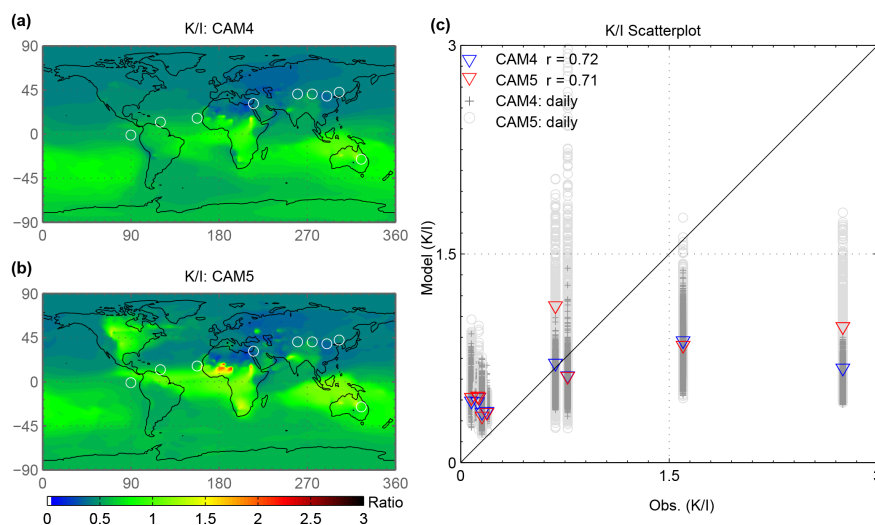
Figure 5. Kaolinite/illite mineral ratio of mineral concentrations near the surface from CAM4 and CAM5 (kg K / kg I) compared to bulk observational ratios (kg K / kg I) from fieldwork by Shen et al. (2005), Glaccum and Prospero (1980), Prospero and Bonatti (1969), Caquineau et al. (1998), Kiefert et al. (1996) and Falkovich et al. (2001). Colored values in (c) represent averages for the month in which the observations occurred, while the grey symbols represent daily averaged values over the course of the simulations (2006–2011).
