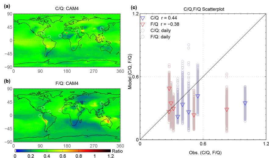
Figure 6. Calcite/quartz and feldspar/quartz mineral ratio comparison of mineral concentrations near the surface from CAM4 (e.g., kg C / kg Q) to bulk observational ratios from fieldwork by Glaccum and Prospero (1980), Prospero and Bonatti (1969), Kiefert et al. (1996), Falkovich et al. (2001) and Shi et al. (2005). Bright blue and red symbols in (c) represent averages for the month in which the observations occurred, while the pale red and blue symbols represent daily averaged values over the course of the simulations (2006–2011).
