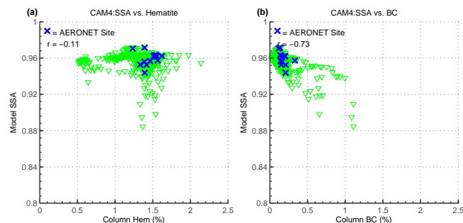
Figure 10. Model single scattering albedo at grid cells with AOD_{\text{dust}} > 0.5 \cdot AOD_{\text{total}} in CAM4 mineralogy is compared to total percent column hematite (a) and total percent column black carbon (b). The locations of AERONET sites used in the comparison in Fig. 9 are plotted in blue.
