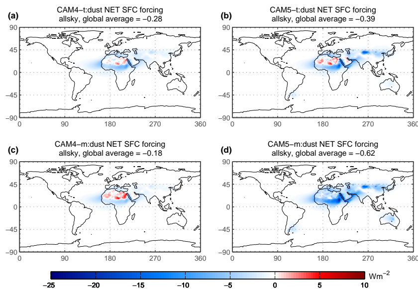
Figure 12. Spatial distribution of annual all-sky radiative forcing (SW + LW) at the surface for CAM4 with tuned dust and with mineralogy (a, c) and for CAM5 with tuned dust and mineralogy (b, d).
