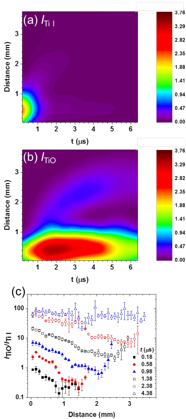
Figure 6. Distance-time contour maps of (a) I_{TiI} and (b) I_{TiO} emission intensities obtained for sample position, OF2 (3.2 mm after the laser focus) (c) The ratio of I_{TiO}/I_{TiI} as a function of distance for different delay times, t . For shorter delay times, t < 1 \mu s, the ICCD detection gate width was set to 0.2 \mu s. For the longer t \geq 1 \mu s, the gate width was set to 1 \mu s.
