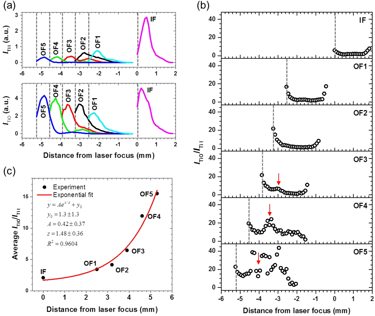
Figure 8. Atomic and molecular emission at different distances from the laser focus: (a) I_{Ti I} and I_{Ti O} profiles as a function of distance, (b) I_{Ti O}/I_{Ti I} profiles spatially and (c) averaged I_{Ti O}/I_{Ti I} ratio. In (a) and (b), the vertical dashed lines indicate the sample surface positions. The arrows in (b) show the gap positions between the two split parts of the fs laser-induced plasma for OF3 , OF4 , and OF5 . These data were obtained with a 1- \mu s ICCD detection gate width delayed from the laser pulse by 1 \mu s.
