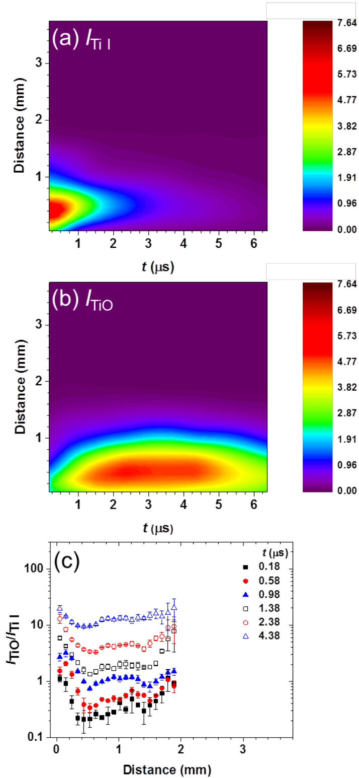
Figure 4. Distance-time contour maps of (a) I_{TiI} and (b) I_{TiO} intensities obtained for sample position, IF (c) The ratio of I_{TiO}/I_{TiI} as a function of distance for different delay times, t . For shorter delay times, t < 1 \mu s , the ICCD detection gate width was set to 0.2 \mu s . For the longer t \geq 1 \mu s , the gate width was set to 1 \mu s . Distance 0 is at the sample surface.
