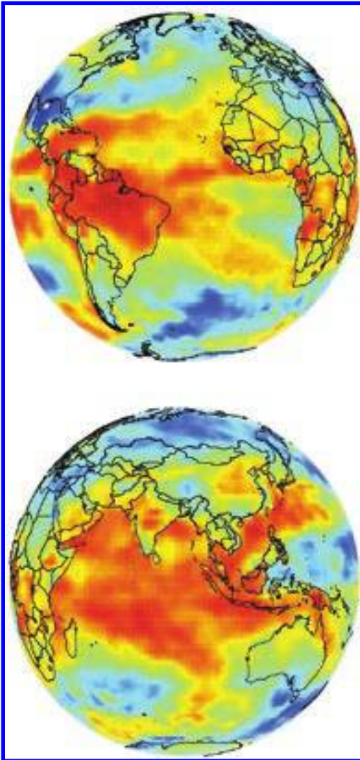
FIGURE 2. CORRELATION BETWEEN DECEMBER SEA SURFACE TEMPERATURE IN THE TROPICAL WEST PACIFIC OCEAN AND TEMPERATURES AT EACH LOCATION FIVE MONTHS LATER
