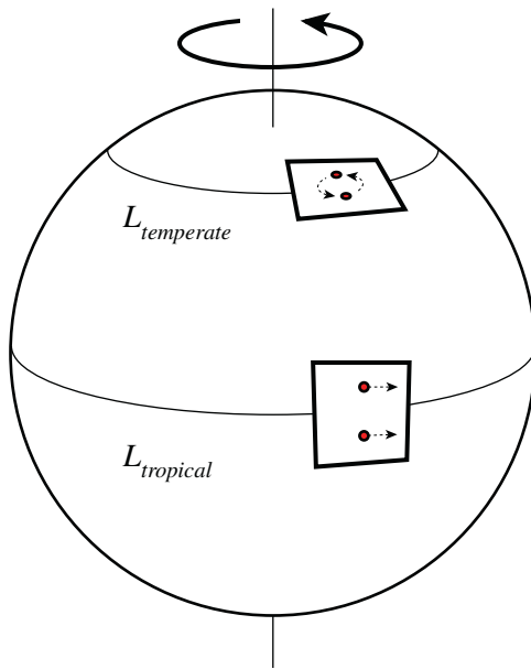
FIGURE 1. TROPICAL LATITUDES EXPERIENCE THE EARTH'S ROTATION DIFFERENTLY FROM TEMPERATE LATITUDES
