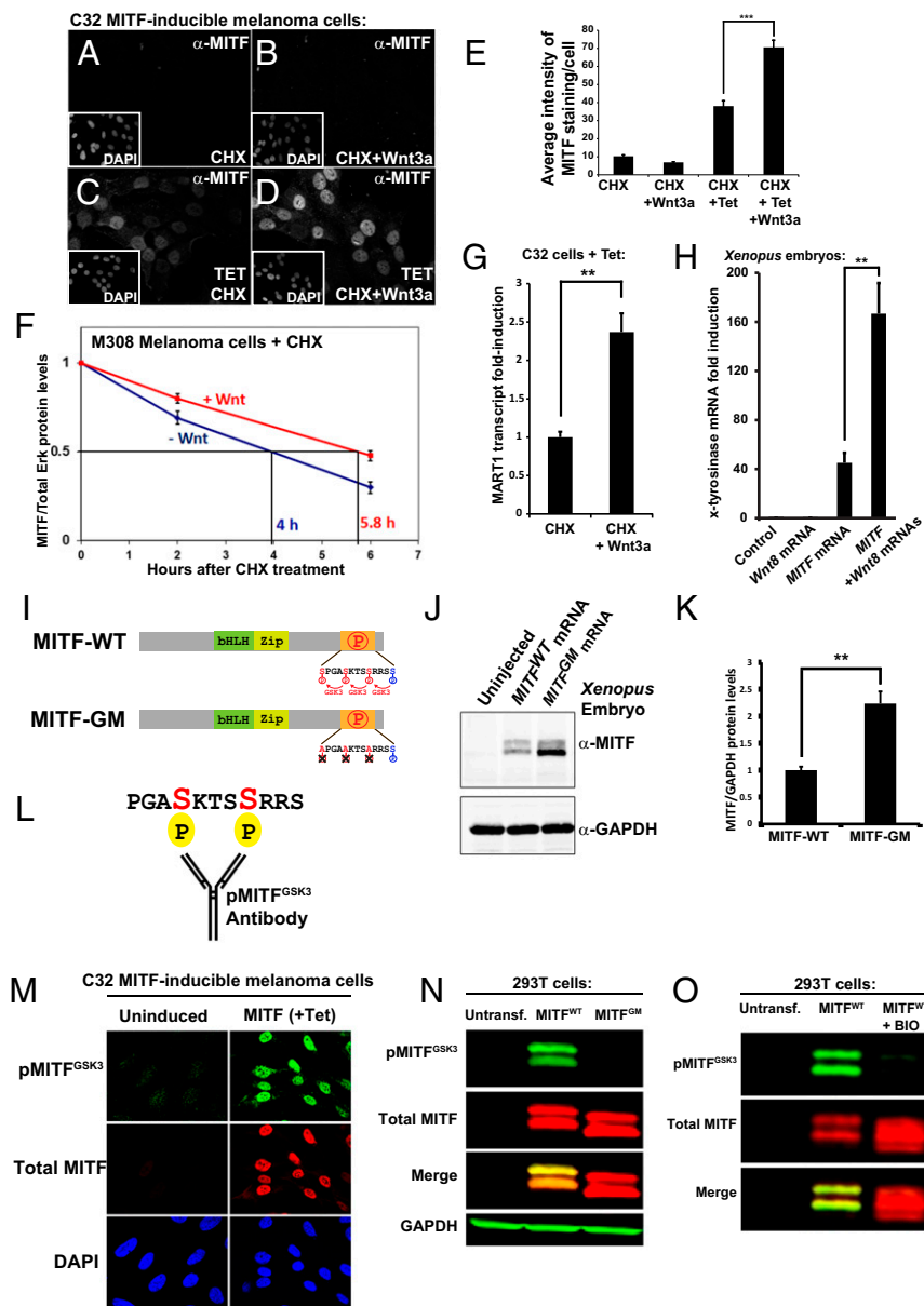
Fig. 5. MITF protein stabilization by Wnt via novel C-terminal GSK3 phosphorylation sites. ( A–D ) MITF immunostainings in C32 cells using a 40 \times objective. Wnt3a protein treatment for 5 h stabilized MITF protein in the presence of CHX. ( E ) Quantification of MITF staining per nucleus from a previous experiment ( ***P < 0.001 ). ( F ) MITF protein levels (normalized to total Erk1/2) from three independent Western blot experiments upon treatment of M308 melanoma cells with Wnt3a; Wnt prolongs the half-life of endogenous MITF protein. ( G ) RT-qPCR of the MITF target gene MART1 in Tet-induced C32 cells treated with CHX and Wnt3a ( **P < 0.01 ). ( H ) RT-qPCR for the MITF target gene x-tyrosinase obtained from Xenopus laevis embryos microinjected with Wnt8 , MITF , or MITF + Wnt8 mRNAs. Wnt8 markedly increased MITF activity ( **P < 0.01 ). ( I ) Diagram depicting MITF wild-type (MITF-WT) and a MITF GSK3 phosphorylation-resistant mutant (MITF-GM). ( J ) Western blot of Xenopus laevis embryos injected with equal amounts of mRNA for MITF-WT or MITF-GM and blotted for MITF. GAPDH was used as a loading control. ( K ) Quantification of Western blots from three independent Xenopus experiments showing that MITF-GM is more stable than MITF-WT ( **P < 0.01 ). ( L ) Diagram of a pMITF GSK3 antibody raised against the indicated peptide corresponding to the C-terminal region of MITF with two phosphorylations. ( M ) pMITF GSK3 antiserum mirrors the total MITF immunostaining pattern detected with an anti-MITF mAb in Tet-induced C32 cells. This indicates that the phospho-antiserum is specific for MITF. ( N ) Western blot of HEK 293T cells transiently transfected with MITF-WT or MITF-GM and blotted for pMITF GSK3 , total MITF, and GAPDH as a loading control. Note that MITF-GM is not recognized by the phospho-specific MITF antibody. ( O ) Western blot of HEK 293T cells transiently transfected with MITF-WT treated with or without BIO, a specific GSK3 inhibitor. Note that pMITF GSK3 , but not total MITF (anti-MITF mAb), is inhibited by BIO.
