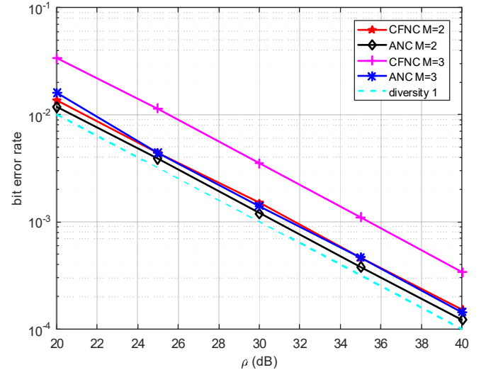
Fig. 4. Bit error rate performance of ANC and CFNC.
