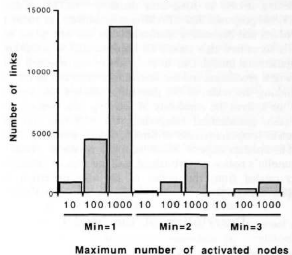
Figure 3: Number of similarity links that are learned by the program, as a function of the maximum number of nodes activated and the minimum number of shared test-links to create a similarity link.
