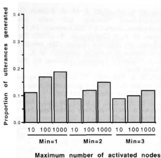
Figure 4: Proportion of the utterances from the mother's sample that are generated by the program, as a function of the maximum number of nodes activated and the minimum number of shared test-links to create a similarity link.
