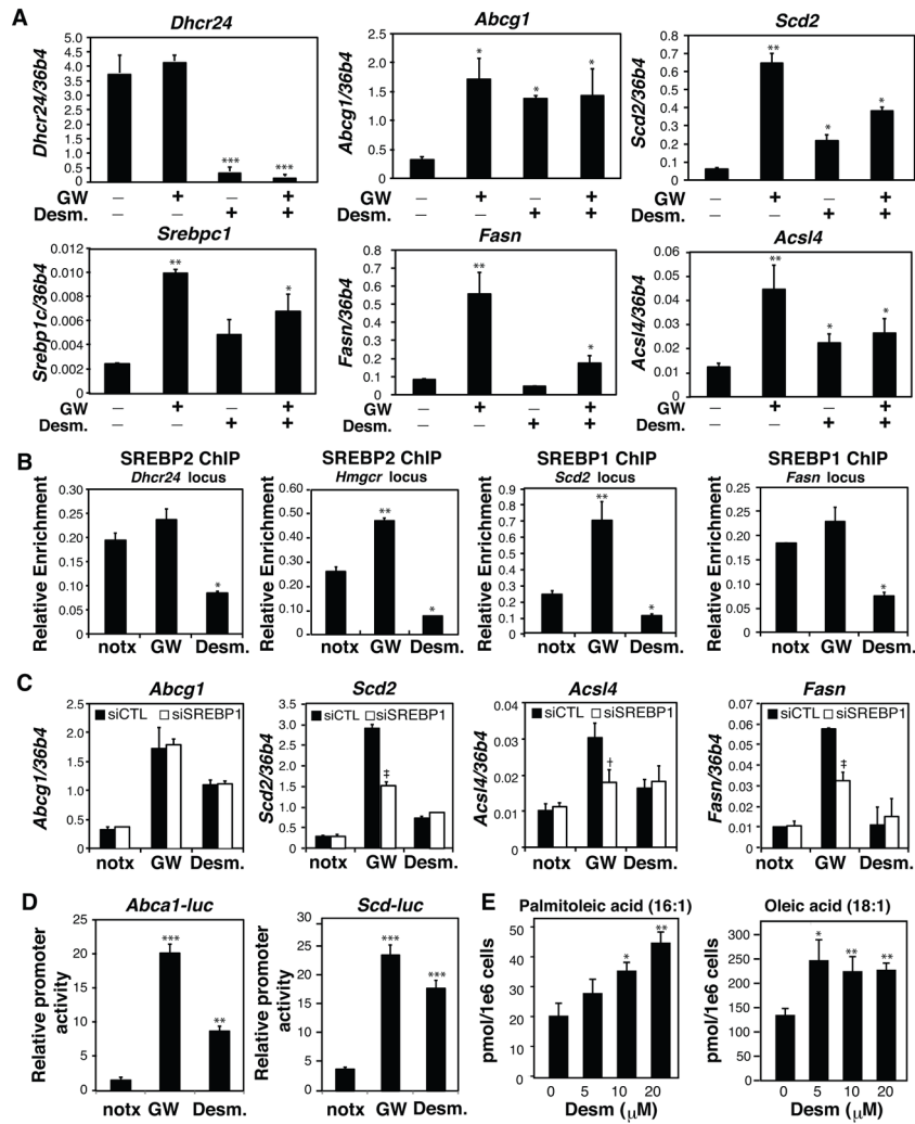
Figure 4. Desmosterol coordinately regulates LXR- and SREBP-dependent gene expression and induces synthesis of palmitoleic and oleic acid in macrophages
