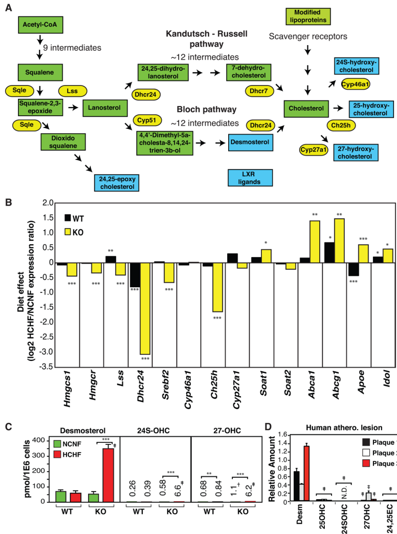
Figure 2. Foam cell formation is associated with increased cellular content of desmosterol A. A simplified scheme of cholesterol and oxysterol biosynthetic pathways. Selected lipid intermediates are labeled in green boxes and important enzymes are labeled in yellow ellipses. Lipid species shown in blue boxes are LXR agonists. B. Effect of the HCHF diet on levels of mRNA transcripts of proteins involved in cholesterol homeostasis from WT and LDLR KO macrophages as determined by microarray analysis. ***P<0.001, **P<0.01, *P<0.05 (n=5). C. Cellular levels of selected endogenous LXR ligands. P-value notations are the same as Figure 1A (n=9). D. Levels of selected LXR ligands in human atherosclerotic lesions. Ligand levels per sample were normalized to cholestanol. Ligand vs. Desmosterol: ***P<0.001, **P<0.01, *P<0.05 (n=3). Error bars represent SEM.
