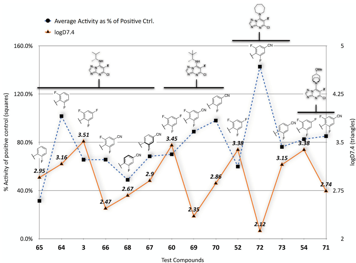
Figure 5. Comparison of selected compounds based on experimental logD 7.4 values (triangles) and MT-stabilizing activity (squares) expressed as the average activity in the AcTub assay at 1 and 10 \mu M normalized to positive control ( i.e. , 100 nM 5 ). LogD 7.4 values were determined via shake flask method (experiments run by Analiza, Inc.)
