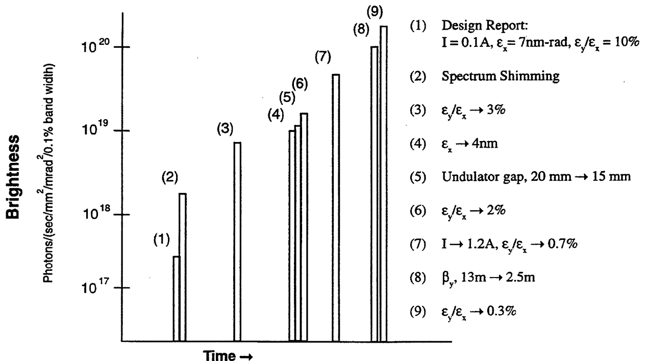
Figure 4. Improvements in ESRF Brightness from 1992 to Present
