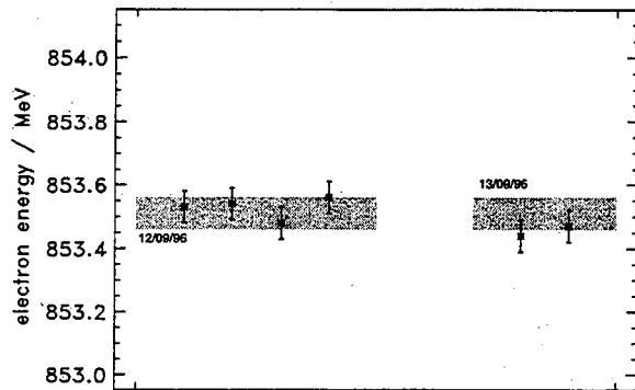
Figure 2. Electron energy measured by resonant spin depolarization (■) and by Compton back scattering
