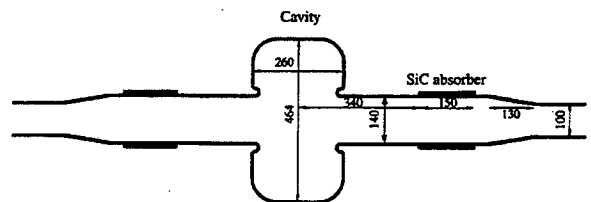
Figure 1. HOM-Damped Cavity for the PF
