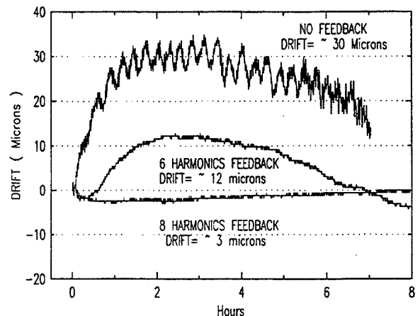
Figure 3. Stabilization of the vertical orbit in the NSLS X-Ray Ring using the harmonic correction algorithm
