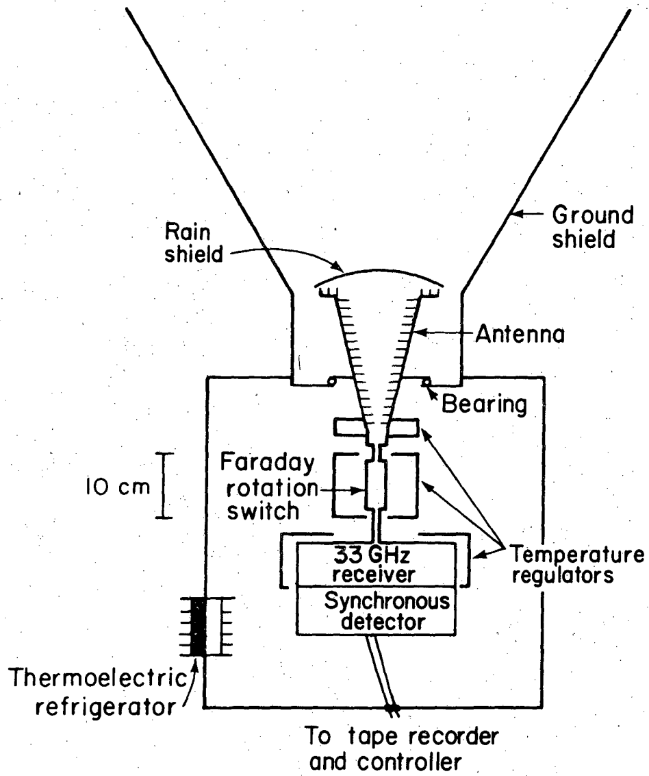
Figure 2. Schematic of microwave polarimeter used.
