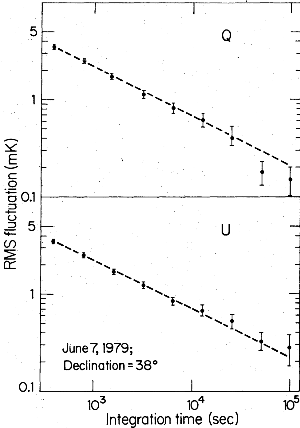
Figure 6. RMS fluctuations versus integration time. 1/t^{1/2} line is drawn in for comparison.
