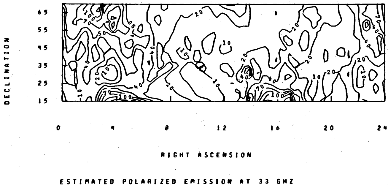
Figure 8. Contour map of estimated polarized galactic synchrotron emission at 33 GHz based upon the survey of Brouw and Spoelstra (1976). Levels are in microKelvin.
