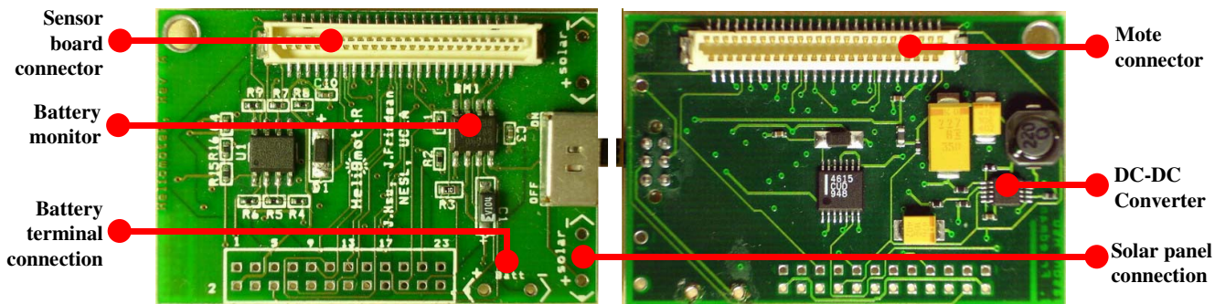
Fig. 4. Top and bottom sides of the Heliomote board.
