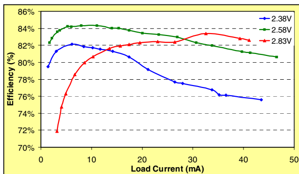
Fig. 5. Efficiency of the Heliomote board as a function of load current at different supply voltages.
