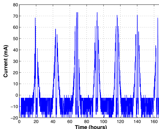
Fig. 6. Plot of battery charging current vs. time
