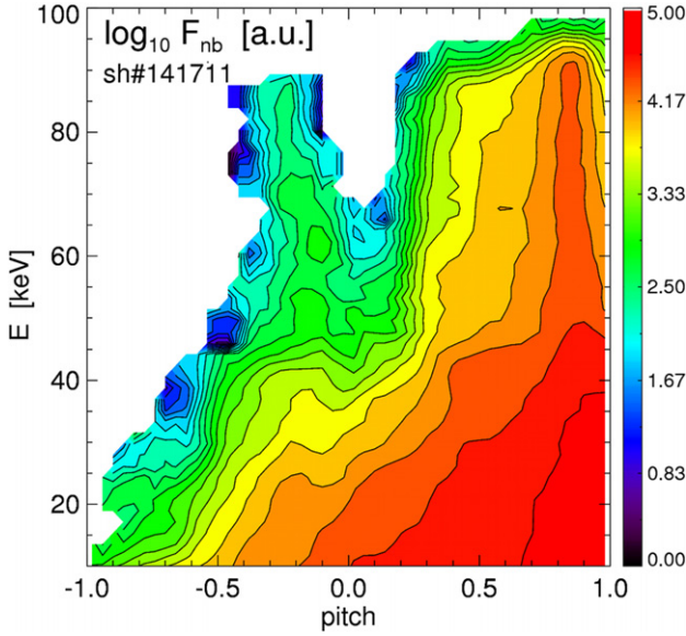
Figure 20. Fast ion distribution as a function of energy and pitch from TRANSP/NUBEAM [36] for discharge no. 141711, t = 470 ms and R \approx 120 cm.
