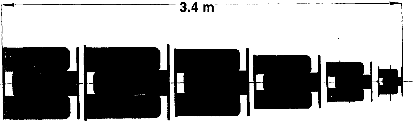
STRAIGHT MATCHING SECTION FOR THE 2MeV ESQ-INJECTOR WARP-3D SIMULATION
