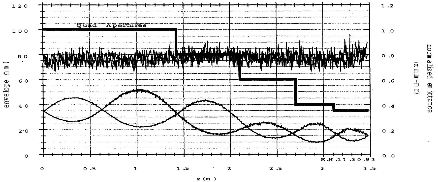
STRAIGHT MATCHING SECTION FOR THE 2MeV ESQ-INJECTOR WARP-3D SIMULATION
