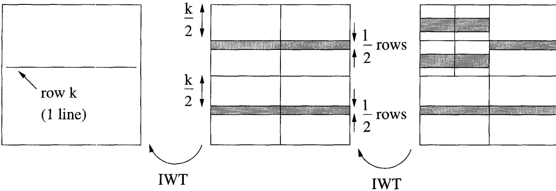
Figure 1: On the left, the printer is ready to print out row k of the output image. The middle picture shows strips of wavelet coefficient rows that are required at the first level of decomposition. On the right are strips required at the second level of decomposition.
