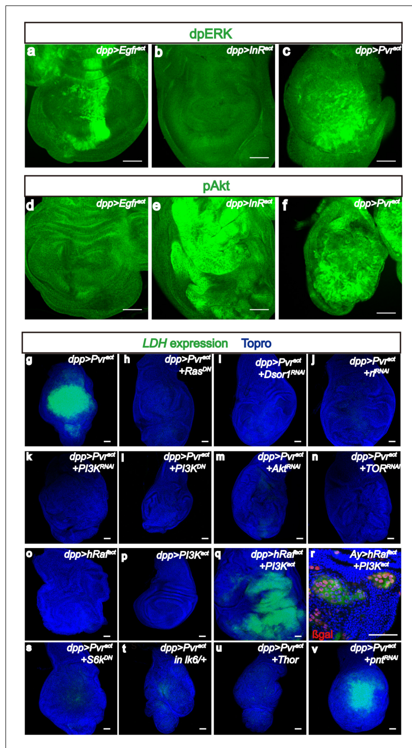
Figure 3. Downstream of Pvr^{act} , ERK and PI3K pathways control Sima translation. All wing discs shown are from wandering third instar larvae. All transgenes are expressed using the dpp^{blk-1} -Gal4 driver. Scale bars, 50 \mu m. (a–f) Differential activation of ERK and PI3K pathways by RTKs. Phospho-specific antibodies against dp-ERK (a–c, green) or p-Akt (d–f, green) are used to detect activation of the corresponding pathways. (a–c) dp-ERK staining is seen in Egfr^{act} (a) and Pvr^{act} (c) backgrounds, but not upon activation of InR (b). (d–f) In contrast to (a–c), p-Akt is detected upon activation of InR (e) and Pvr (f) but not Egfr (d). Thus only Pvr^{act} causes both the ERK (assayed by ERK phosphorylation) and PI3K (assayed by Akt phosphorylation) pathways to be activated. (g–v) Both PI3K and ERK pathways must be activated for LDH-GFP induction. Expression of LDH-GFP (green) marks glycolytic tissue. In Figure 3 continued on next page
