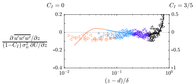
FIG. 4. Ratio of the transport and production terms contributing to the momentum flux in Eq. (6). Gradient-diffusion closure (K-theory), which neglects transport, is valid when the ratio is small. The left vertical axis is based on C_I = 0 (no isotropization) and the right C_I = 3/5 (isotropization predicted by rapid distortion theory).
