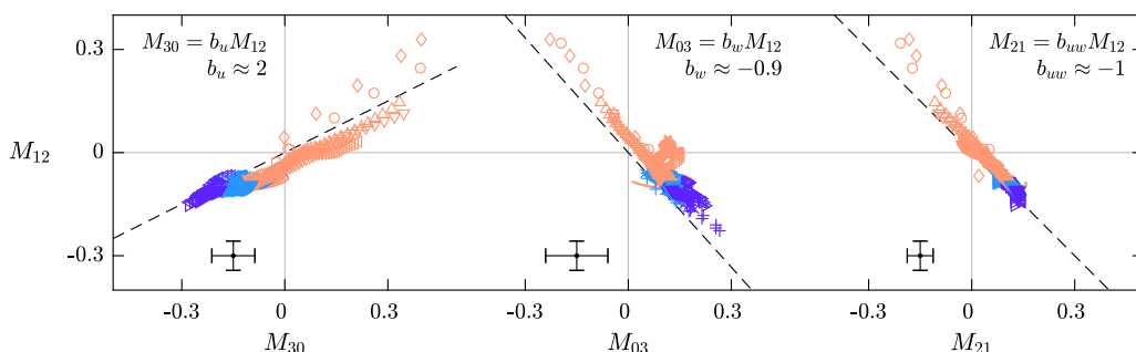
FIG. 7. Linear relations between the third-order moments M_{ij} in the roughness sublayer and logarithmic regions. Dashed lines (---) represent the linear relations given by Raupach [9]. The error bars are estimated 95% confidence intervals for the mesh PIV cases. Data symbols correspond to the cases in Table I.
